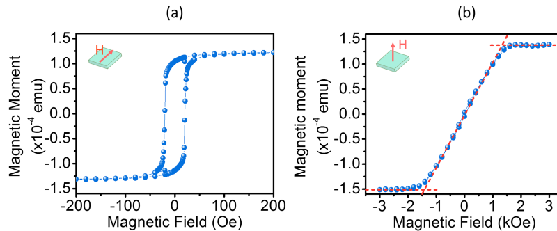
FIG. 3. Static magnetic properties: (a) and (b) show the hysteresis loops measured by a vibrating sample magnetometer using different fields, as indicated. The sample size is 5 mm \times 4 mm. The dashed lines in (b) indicate how the saturation field is determined.
