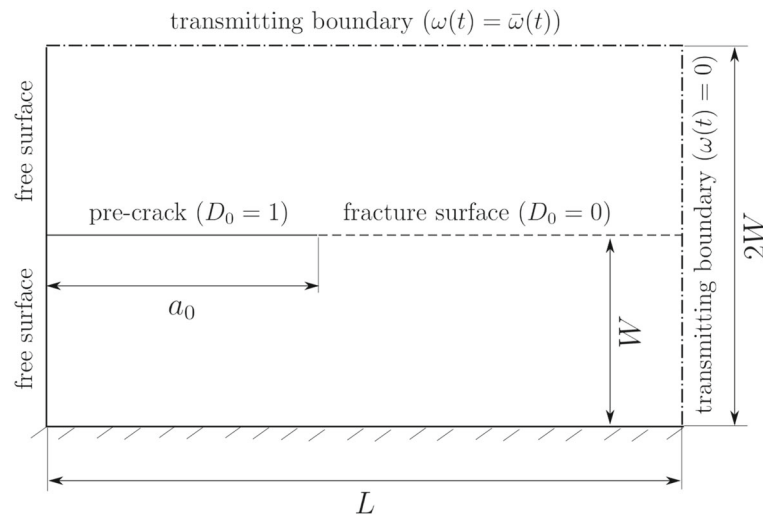
a Computational domain, boundary conditions and fracture surface.
