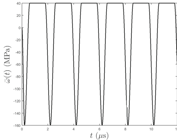
b Characteristic load history on top edge, \bar{\omega}(t) .
