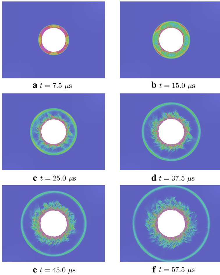
Fig. 8 Solution visualization sequence for explosively loaded wellbore
