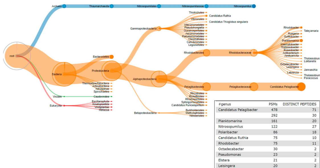
Figure 5. Taxonomy analysis using Unipept. Bacterial PSMs were subjected to Unipept analysis against UniProt database using lowest common ancestor algorithm to generate outputs for taxonomic analysis. These outputs include a Unipept Viewer which is an interactive visualization plugin that can be used to visualize taxonomic distribution of the ocean metaproteomic dataset. Unipept also generates a Comma-Separated Values (CSV) format file that lists the peptide assignments to taxa. That file then can be parsed to generate a tabular output (lower right).
