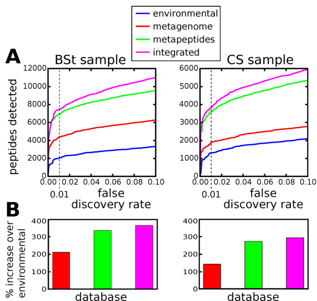
Figure 2. Peptides detected in different searches. (A) Line plots of peptide false discovery rate (FDR, horizontal axis) vs number of peptide sequences detected at that FDR in the Bering Strait (BSt) and Chukchi Sea (CS) samples (vertical axis), when searched four different ways. Dashed line indicates peptide yield at FDR > 0.01 from searches against the NCBI environmental database (2050 in BSt and 1317 in CS), against the metagenome-derived database (4344 and 1877), against metapeptides derived from the sample being searched (6918 and 3606), and integrated results from all three databases (7508 and 3871). (B) Detected peptide counts at FDR < 0.01 in the metagenome, metapeptide, and integrated database searches as a percentage of the counts detected in environmental search.
