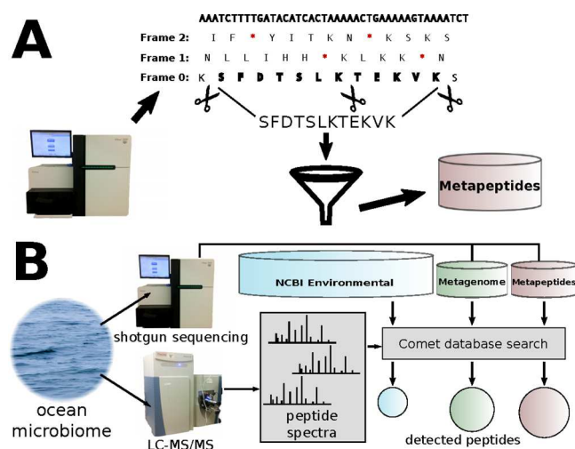
Figure 1. Multiple approaches for metaproteomics of microbiome samples. (A) After high-throughput sequencing, metapeptide database construction begins with six-frame translations of raw sequencing reads, or with gene fragments predicted from reads. Amino acid sequences are trimmed to their outermost tryptic sites to yield metapeptide sequences. Candidate metapeptides are filtered on per-base quality scores, sequence length and other features. Passing candidates are added to the database. (B) Alternative proteomics workflows. Microbiome samples are subjected to shotgun metagenomic sequencing and LC-MS/MS analysis. MS/MS spectra are searched with Comet against the NCBI environmental database, against predicted genes from an assembled metagenome, or against a metapeptide database, resulting in peptide yields of different size. Photographs copyright 2016 Damon May.
