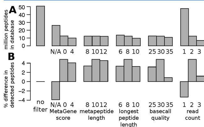
Figure 5. Metapeptide parameter comparison. Comparisons between metapeptide databases constructed with different filtering parameters. The bars on the far left represent a database of MetaGene fragments trimmed to outermost tryptic ends but otherwise are unfiltered. Each group of three bars represents three different values for a single parameter, with all other parameters set as described in section 2.2. In each group, the middle value represents the value used to generate the results described in Figures 2–5. The N/A value for MetaGene score represents the use of raw six-frame translations of reads instead of MetaGene output. (A) Millions of tryptic peptides in each database. (B) Percent difference in counts of peptides detected in a search of 24 000 scans from the three BSt sample replicates at FDR < 0.01 against each database, as compared with search against the unfiltered, trimmed MetaGene database.
