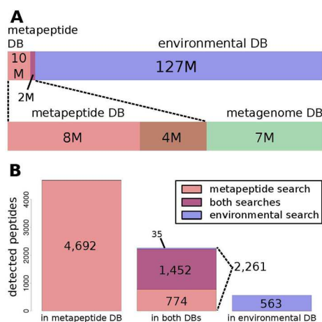
Figure 3. Database and detected peptide comparisons. (A) The BSt metapeptide database contains roughly 12 million tryptic peptides. The environmental database contains 129 million, with an intersection between the two databases of 2 million peptides. The metagenome database contains 11 million peptides, with 4 million peptides in common with the BSt metapeptide database. (B) Searching against the BSt metapeptide database detects 6918 unique peptides at FDR < 0.01, vs 2050 when searching against the environmental database, with 1452 in common. Of the 2261 peptides detected in either search that were present in both databases, 1452 were detected in both searches, 774 were only detected in the BSt metapeptide database search, and 35 were only detected in the environmental database search.
