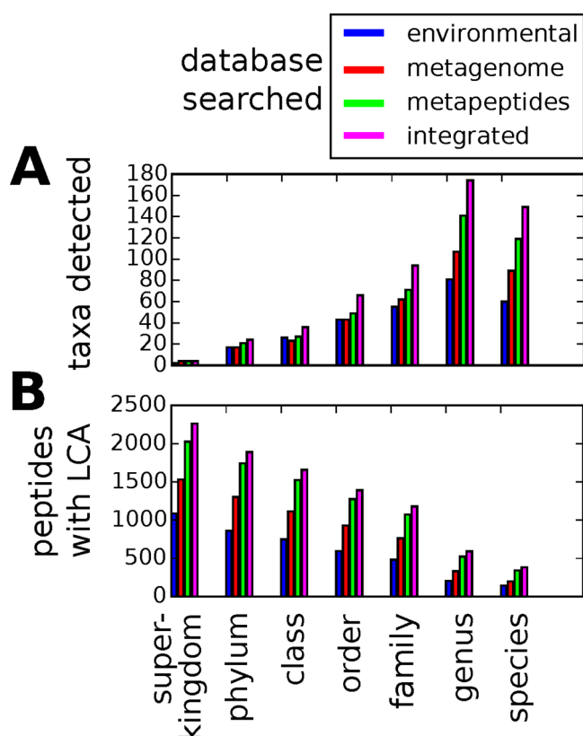
Figure 4. Taxonomic inference summary. Bar charts comparing the taxonomic information derived from four different searches of the BSt sample: against the NCBI environmental database, against the metagenome-derived database, against site-specific metapeptides, and integrating results from all three databases. (A) Counts of taxa detected, by rank from superkingdom to species. (B) Counts of peptides associated with an LCA at each rank.
