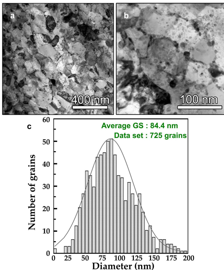
Figure 1. a) Low magnification (scanning) transmission electron microscopy (S)TEM Bright Field (BF) image of as-received (i.e., post-ECAE processed) sample showing grain structure. b) High magnification STEM BF TEM image showing the high density of Ta-based clusters residing in the lattice as well as along the grain boundaries of the Cu-based matrix. c) Grain size distribution plot of the ECAE processed sample.
