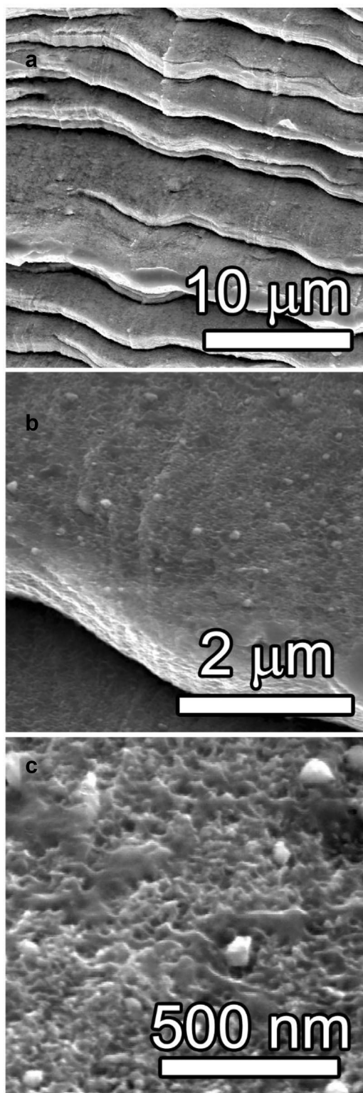
Figure 7. a, b, c) SEM micrographs of progressively increased magnification showing the pleated surface of a machining chip from stabilized nanocrystalline Cu-3Ta.
