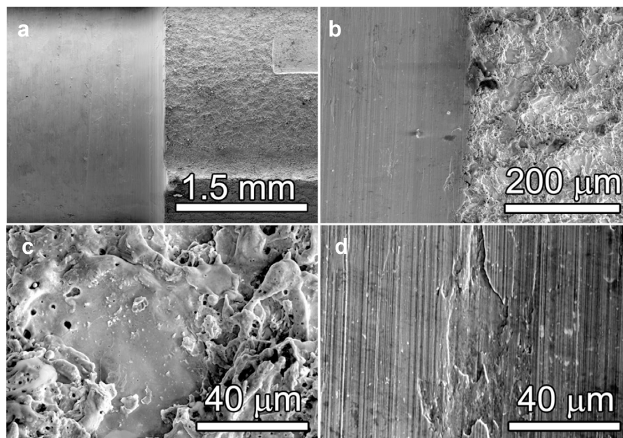
Figure 4. Difference in surface appearance resulting from the lathing and EDM cutting. a, b) Low and medium magnification SEM images of the lathed surface (left side) and EDM surface (right side). c, d) High magnification SEM images of the EDM surface c) and the lathed surface d).
