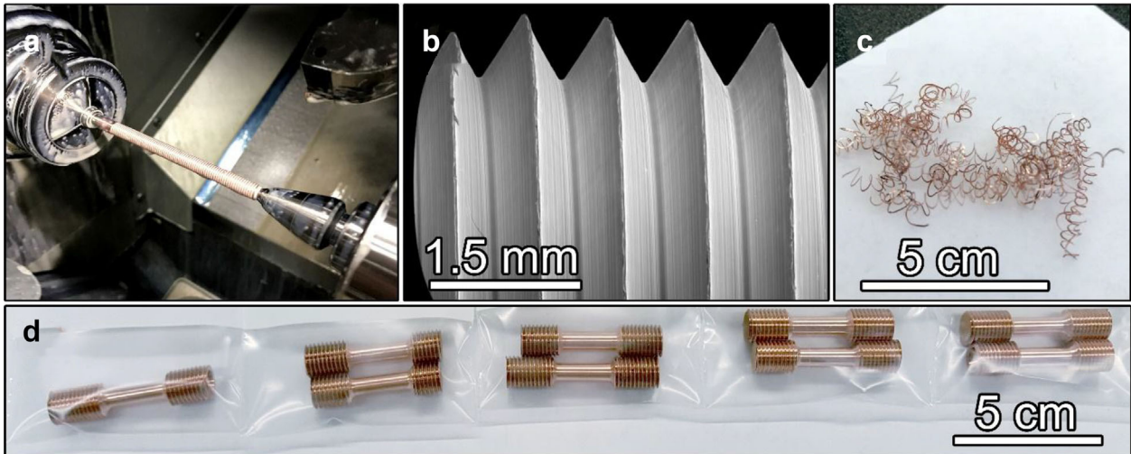
Figure 3. Threading process. a) Image of the core still in the lathe after being turned and threaded to the appropriate dimensions. b) SEM image showing the respective surface finish of individual threads. c) Representative turning from the machining process. d) Numerous tensile samples showing uniformity and reproducibility of the machining process for Cu-3Ta.
