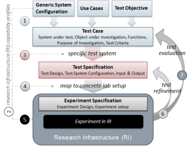
Fig. 1. The main steps in the ERIGrid methodology for holistic testing.
