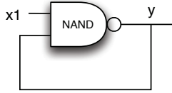
Figure 3: A circuit with oscillation.
