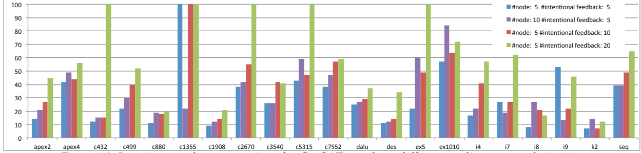
Figure 10: Iteration number comparison for CycSAT attack on different cyclic encrypted circuits.
