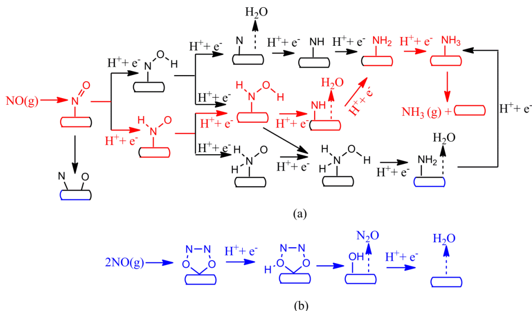
Scheme 1: Schematic depiction of the pathways of NO electrochemical reduction on the Co-N 4 /graphene surface at (a) low and (b) high coverages. The preferred pathways are plotted in red (for low coverage) and blue (for high coverage) lines.
