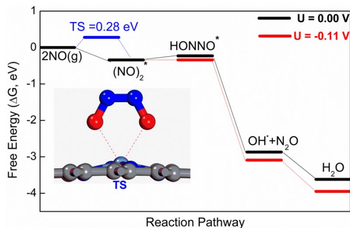
Fig. 7. Free-energy diagrams for the NOER on Co-N 4 /graphene at high coverages along the most energetically favorable pathway at pH=0 and at zero or onset potential. TS is the transition state of the rate-determining step ( 2\text{NO}(\text{g}) \rightarrow (\text{NO})_2^* ). The activation barriers for other steps (not shown in the figure) are 0.19, 0.09, and 0.00 eV, respectively, for (\text{NO})_2^* \rightarrow \text{HONNO}^* \rightarrow \text{N}_2\text{O}(\text{g}) + \text{OH}^* \rightarrow \text{N}_2\text{O}(\text{g}) + \text{H}_2\text{O}(\text{l}) .
