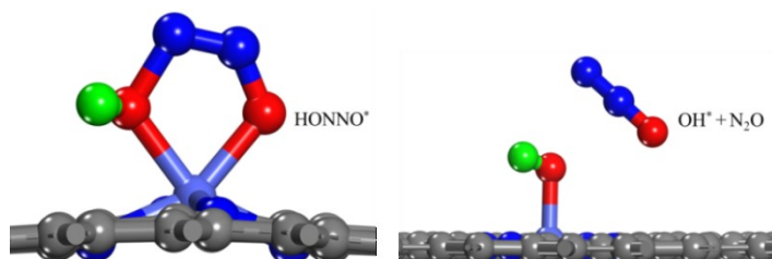
Fig. 6. The optimized geometric structures of key intermediates ( HONNO^* and OH^* ) along the reaction path of NOER proceeded on Co- N_4 /graphene at high coverages.
