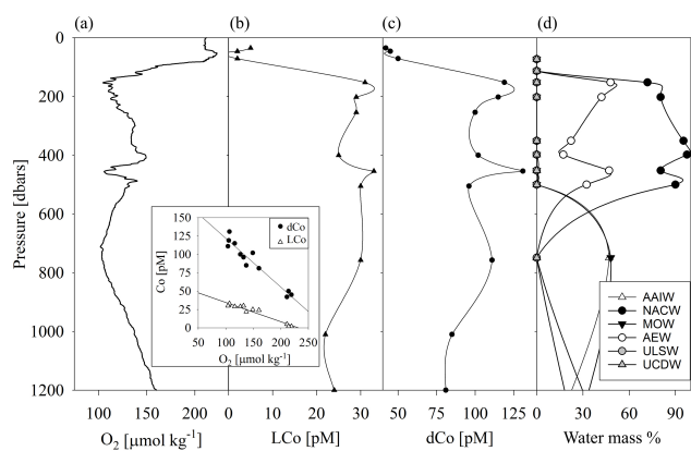
Figure 14. Intermediate depth profile for (a) O_2 , (b) labile cobalt (c) total cobalt and (d) water mass as a percent for USGT10-07. A strong linear correlation with O_2 is observed (inset). A small but distinct maximum is observed between 400 and 600 m and demonstrates the capability of water mass features to influence the cobalt vertical profile at these depths.
