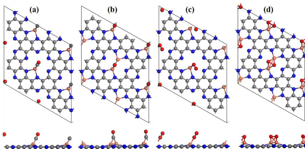
Figure 3. Top and side views of CO adsorption on \text{Cu}_1@\text{C}_2\text{N} (a) and \text{Cu}_2@\text{C}_2\text{N} (b), and \text{O}_2 adsorption on \text{Cu}_1@\text{C}_2\text{N} (c) and \text{Cu}_2@\text{C}_2\text{N} (d). Color scheme: Cu, orange; C, gray; N, blue; O, red.
