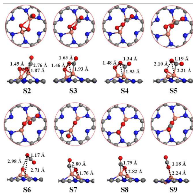
Figure 7. Atomic configurations of S2-S9 and the key structural parameters for CO oxidation via L-H mechanism on \text{Cu}_2@\text{C}_2\text{N} . The corresponding energy profiles are given in Figure 6 as marked in red. Color scheme: C, gray; N, blue; O, red; Cu, orange.
