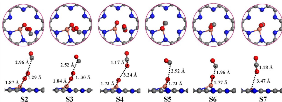
Figure 5. Atomic configurations of S2-S7 and the key structural parameters for CO oxidation via E-R mechanism on \text{Cu}_1@\text{C}_2\text{N} . The corresponding energy profiles were given in Figure 6 as marked in pink. Color scheme: C, gray; N, blue; O, red; Cu, orange.
