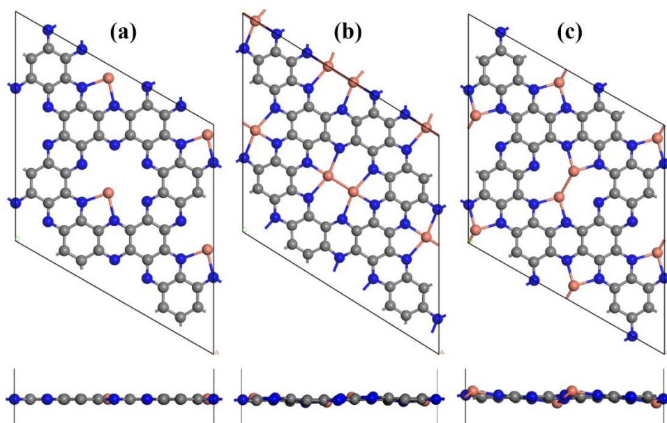
Figure 2. Top and side views of the 2 \times 2 \text{Cu}_1@\text{C}_2\text{N} with Cu at P2 site (a), \text{Cu}_2@\text{C}_2\text{N} with \text{Cu}_2 at P1P1 site (b), and \text{Cu}_2@\text{C}_2\text{N} with \text{Cu}_2 at P2P2 site (c). Color scheme: Cu, orange; C, gray; N, blue.
