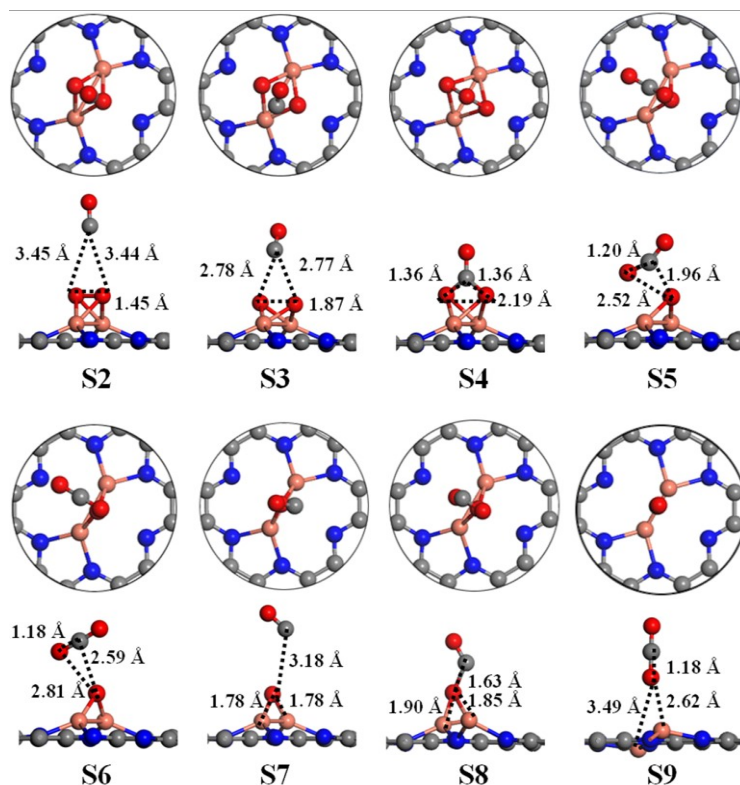
Figure 8. Atomic configurations of S2-S9 and the key structural parameters for CO oxidation via E-R mechanism on Cu 2 @C 2 N. The corresponding energy profiles were given in Figure 6 as marked in black. Color scheme: C, gray; N, blue; O, red; Cu, orange.
