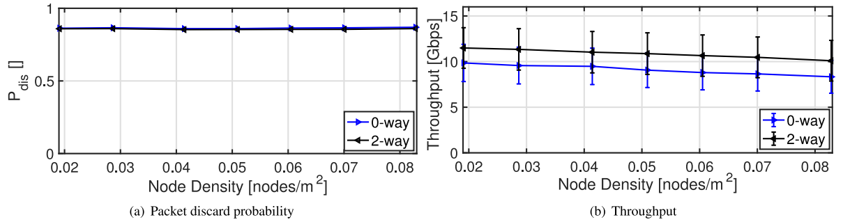
Fig. 8. Performance of MAC protocols in macroscale centralized scenario.
