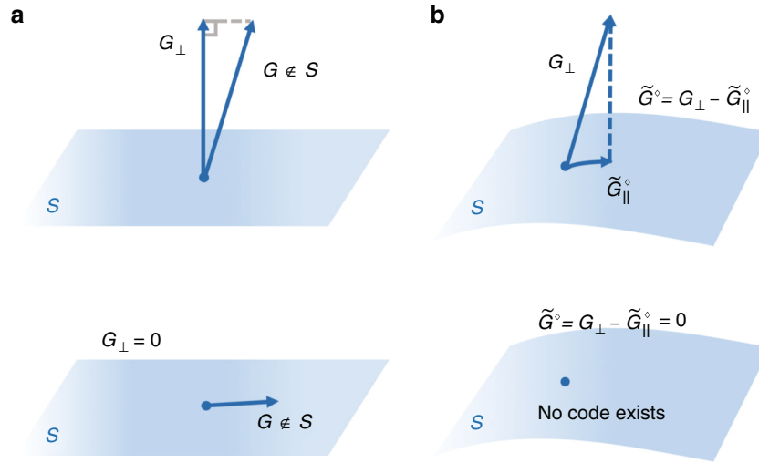
Fig. 2 Schematic illustration of HNLS and code optimization. a G_{\perp} is the projection of G onto S in the Hilbert space of Hermitian matrices equipped with the Hilbert-Schmidt norm \sqrt{\text{tr}(O \cdot O)} . G_{\perp} \neq 0 if and only if G \notin S , which is the HNLS condition. b \tilde{G}^{\diamond} is the projection of G onto S in the linear space of Hermitian matrices equipped with the operator norm \|O\| = \max_{|\psi\rangle} \langle \psi|O|\psi \rangle . In general, the optimal QEC code can be constructed from \tilde{G}^{\diamond} and \tilde{G}^{\diamond} is not necessarily equal to G_{\perp} .
