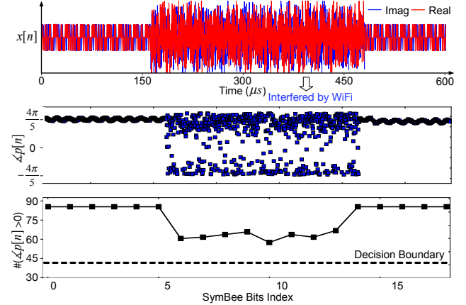
Fig. 20. An example of WiFi interfered SymBee signal and the corresponding number of phase values in the boundary.
