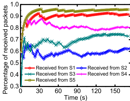
Figure 1. Packet reception under collisions: the percentage of received packets from each sender.
