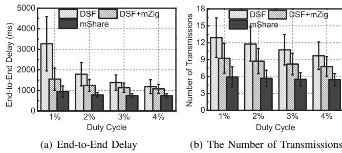
Figure 14. The performance comparison in different duty cycles.
