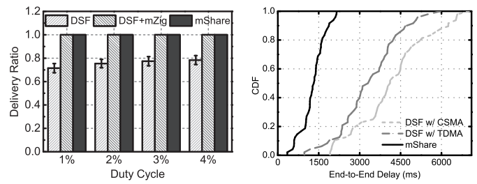
Figure 15. Comparison with TDMA
