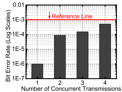
Figure 2. The capability of decoding concurrent transmissions
