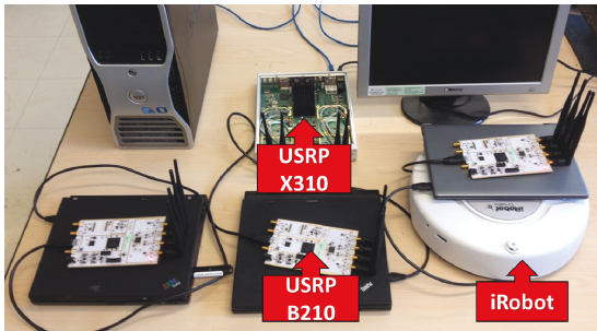
Figure 8. USRP testbed
