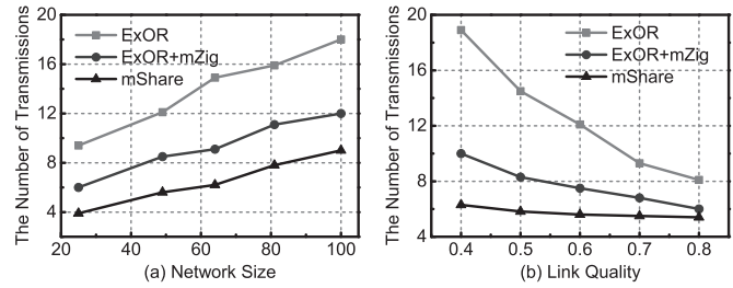
Figure 17. The performance comparison under different (a) network sizes and (b) link qualities in opportunistic routing.
