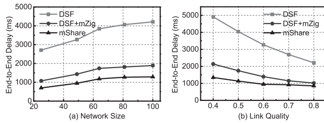
Figure 16. The performance comparison under different (a) network sizes and (b) link qualities in data collection.
