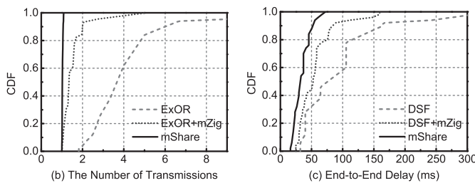
Figure 11. mShare performance in opportunistic routing
