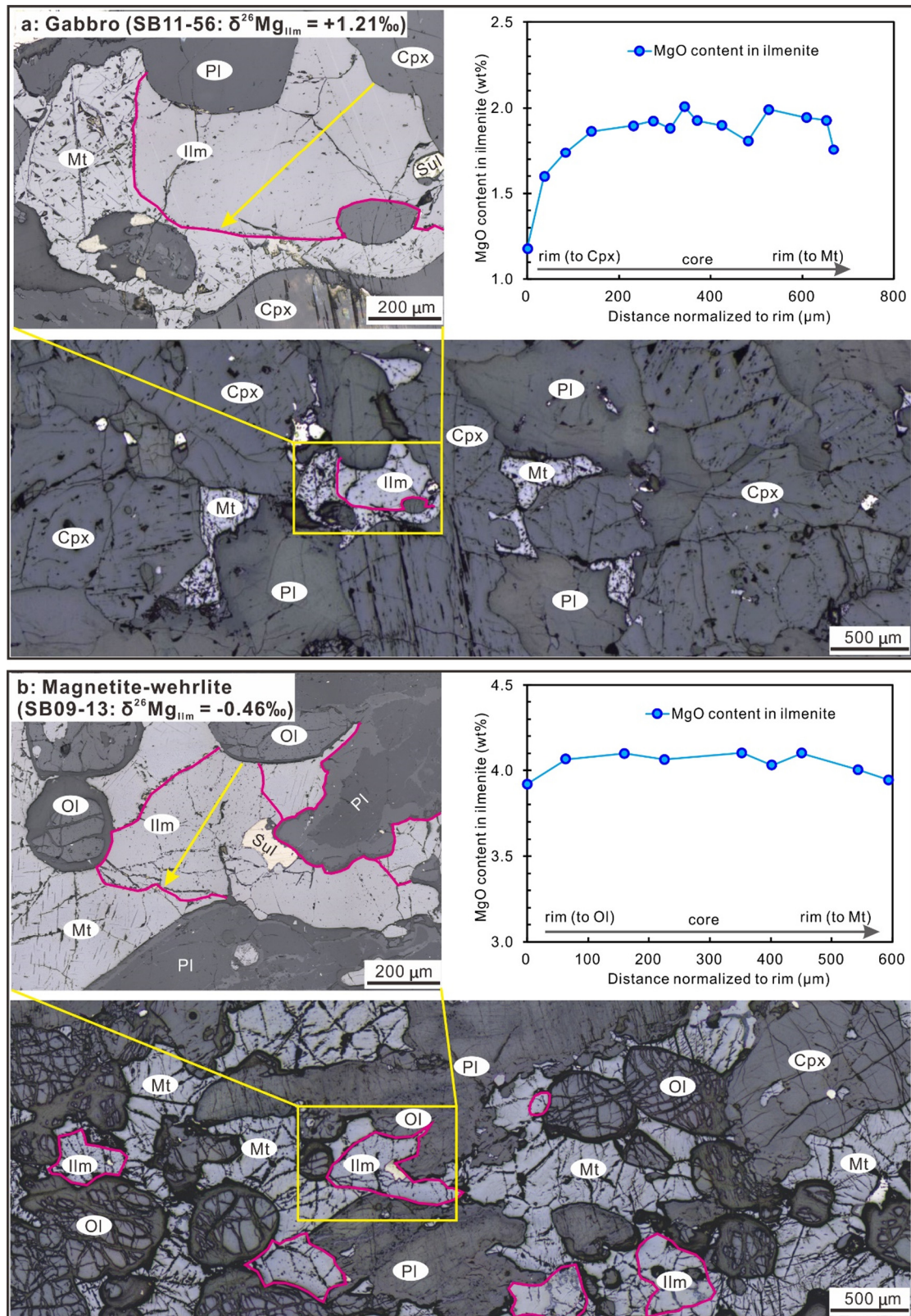
Fig. 1. (a) MgO contents in ilmenite along a traverse in the gabbro, showing decrease of MgO concentration from the core to the rim in contact with ferromagnesian silicates; (b) MgO contents in ilmenite along a traverse in the magnetite-wehrlite, showing constant MgO concentration from the core to the rim. The horizontal axis plots distance normalized to the rim in contact with ferromagnesian silicates. Abbreviations: Ol = olivine, Cpx = clinopyroxene, Pl = plagioclase, Ilm = ilmenite, Mt = magnetite, and Sul = sulfide.
