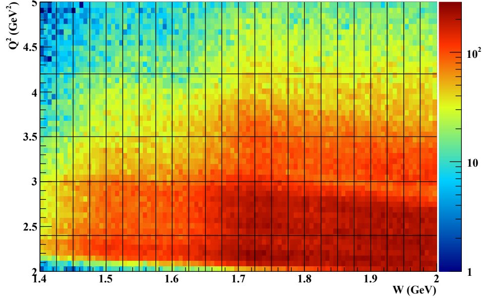
FIG. 8. (Color Online) The kinematic coverage of the p + p events, shown as a scatter-plot as a function of squared 4-momentum transfer Q^2 and center of mass energy W . Bins are shown within which the integrated and nine 1-fold differential p + p cross sections were obtained.
