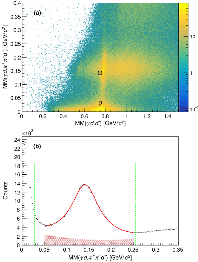
Fig. 2. (a) The y-axis represents the missing mass, Y , in the reaction \gamma d \rightarrow \pi^+\pi^-d' while the x-axis shows the distribution of the missing mass, X , in the reaction \gamma d \rightarrow d' X . (b) Shown is the y-axis projection of (a). The vertical dashed lines represent the position of the missing mass cut made to select \omega -events using the fit shown by the solid curve. An estimate of the possible background shape is shown by the shaded region.
