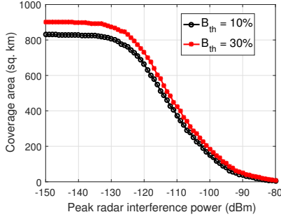
Fig. 7: Effect of radar interference on NB-IoT coverage.
