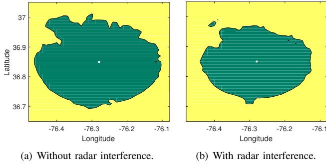
Fig. 6: Coverage area (shown in green) of NB-IoT eNodeB.
