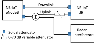
Fig. 3: Block diagram of the experimental setup
