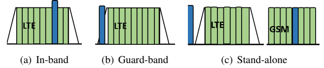
Fig. 1: Three modes of operation of NB-IoT
