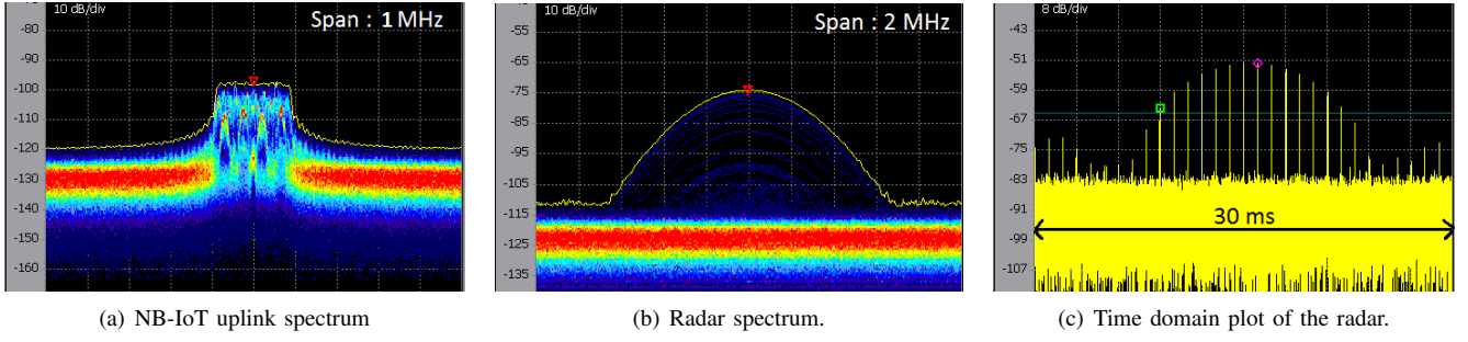
Fig. 2: Plots from the Tektronix spectrum analyzer used as a measurement device in our experiments.
