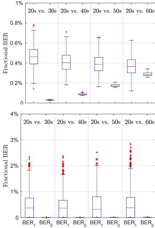
Fig. 8: Fractional Bit Error Rates BER_1 and BER_2 (in %) computed between subsequent decay times for PandaBoard (top) and Galileo (bottom).
