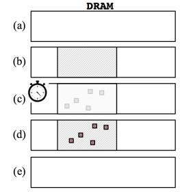
Fig. 2: Five steps required for run-time access of a DRAM PUF. Only during steps (b) – (d) the memory associated with the PUF is not usable for any other processes.
