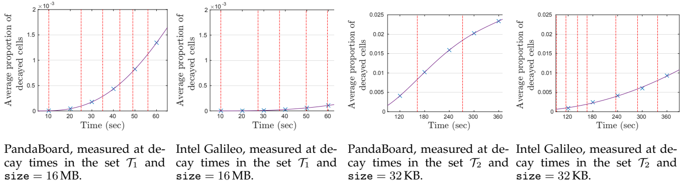
Fig. 4: Proportion of decayed DRAM cells as a function of time for multiple instances of the PandaBoard and the Intel Galileo, (left two graphs) for decay times \mathcal{T}_1 = \{10s, 20s, 30s, 40s, 50s, 60s\} and size = 16 MB and (right two graphs) for decay times \mathcal{T}_2 = \{120s, 180s, 240s, 300s, 360s\} and size = 32 KB. Possible challenge times are indicated by vertical lines.
