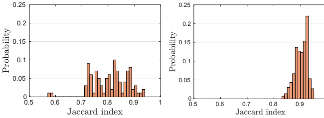
Fig. 7: Distribution of J_{\text{intra}} values computed between measurements pairs, taken at enrollment and reconstruction from the same logical PUF instances, over \approx 16 months apart. Values are shown for the PandaBoard left and Intel Galileo right.
