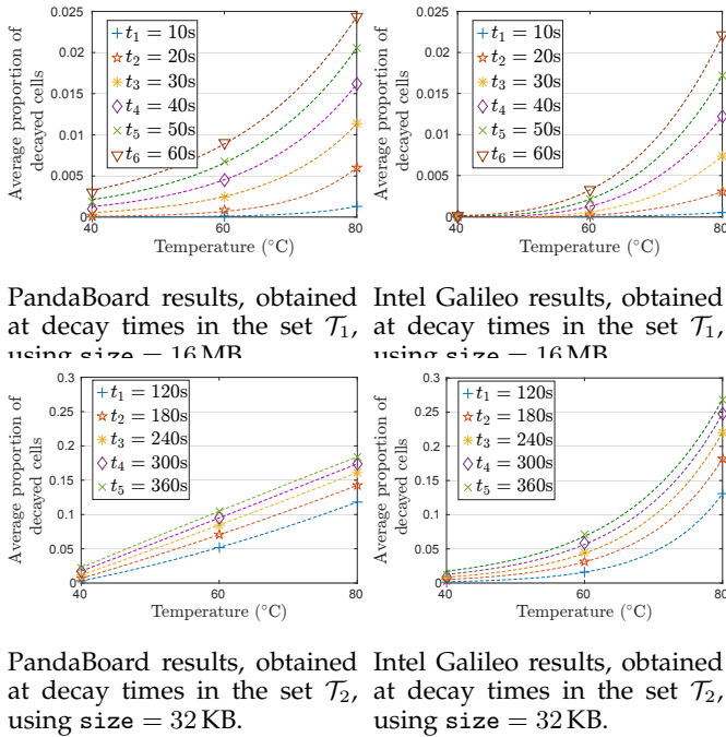
Fig. 5: Proportion of decayed DRAM cells as a function of temperature for multiple instances of the PandaBoard and the Intel Galileo, (top) for decay times \mathcal{T}_1 = \{10s, 20s, 30s, 40s, 50s, 60s\} and size = 16 MB and (bottom) for decay times \mathcal{T}_2 = \{120s, 180s, 240s, 300s, 360s\} and size = 32 KB.
