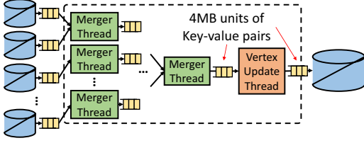
Figure 11: A multithreaded software implementation of sort-reduce
