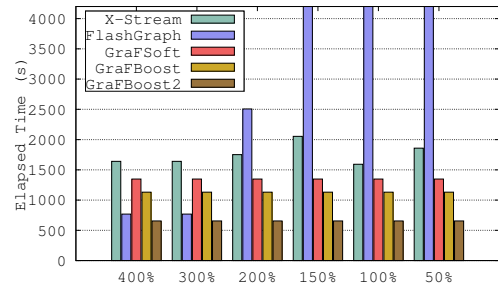
(b) PageRank iteration execution time on machines with various amounts of memory (Lower is faster)
