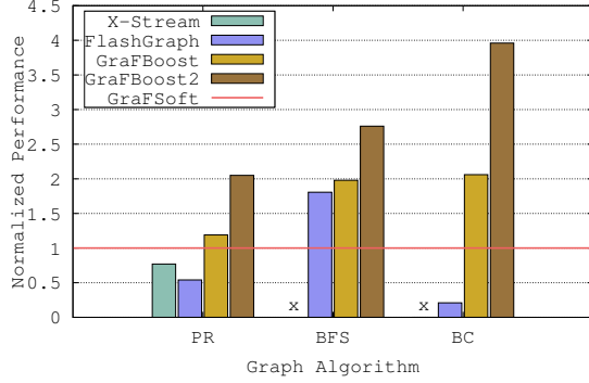
(a) Performance of the algorithms on a machine with 64 GB of memory, normalized to the performance of software GraFBoost (Higher is faster)
