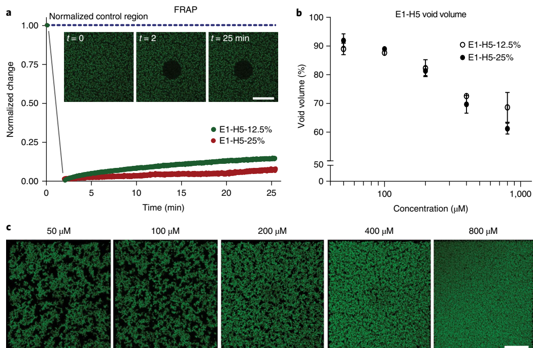
Fig. 5 | Network stability and void volume a , As determined by the limited fluorescence recovery 25 min after bleaching, 12.5% and 25% networks have a high kinetic stability and limited liquid-like properties; Inset pictures are shown for E1-H5-25% at 400 \mu\text{M} . b , Void volumes can be tuned from 60% to 90% by altering polymer concentration. Data represent mean \pm s.e.m. ( n = 4 independent samples). c , Representative 20- \mu\text{m} -thick image stacks are shown for each measured concentration. Scale bars are 50 \mu\text{m} .
