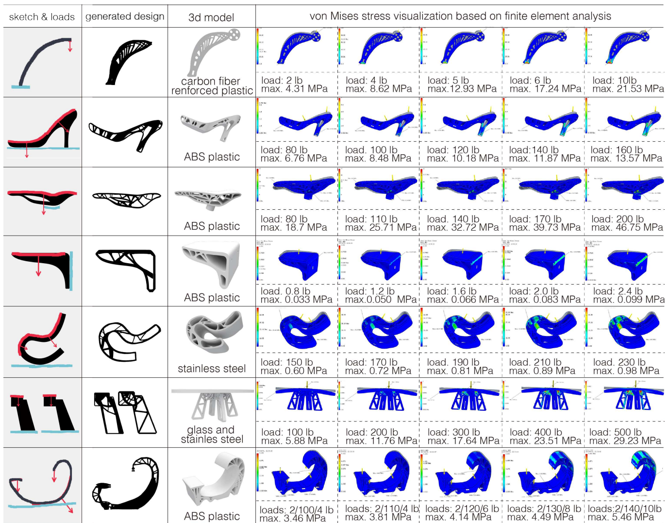
Figure 12. All our fabricated examples from the sketches in Forte, to generated 2D designs, and to post-processed 3D models; we performed a Finite Element Analysis on each 3D model based on the input loading scenario, which shows consistent stress distribution across a range of increasing loads.
