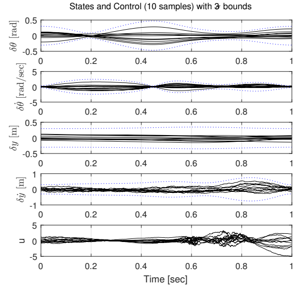
Fig. 1. Linearized Cart-pole states & controls.
