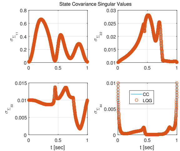
Fig. 2. Linearized Cart-pole: State covariance Singular Values.
