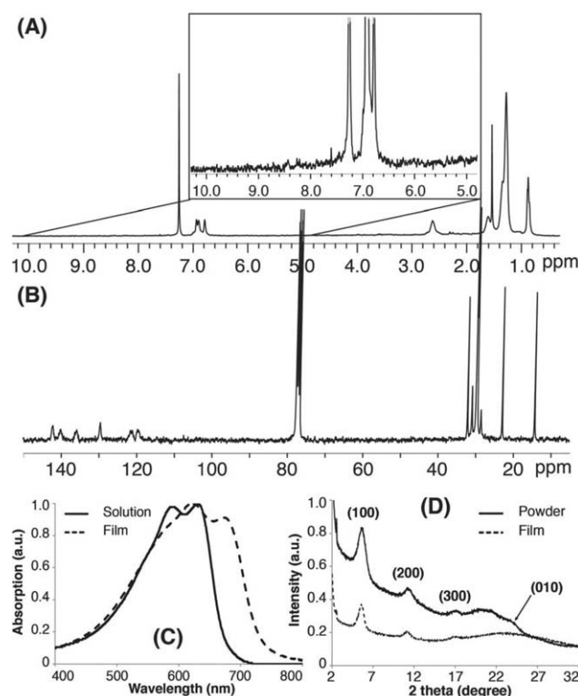
FIGURE 2 (A) ^1\text{H} NMR (300.13 MHz, \text{CDCl}_3 ) spectrum of P3DTV. (B) ^{13}\text{C} NMR (75.48 MHz, \text{CDCl}_3 ) spectrum of P3DTV. (C) UV-Vis absorption spectra of P3DTV in chlorobenzene ( 10^{-5} M repeating units, solid line) and as thin film spin-cast from chlorobenzene solution (dashed line). (D) X-ray scattering profiles of P3DTV as powder (solid line) and as thin film spin-cast from chlorobenzene solution (out-of-plane, dashed line).
