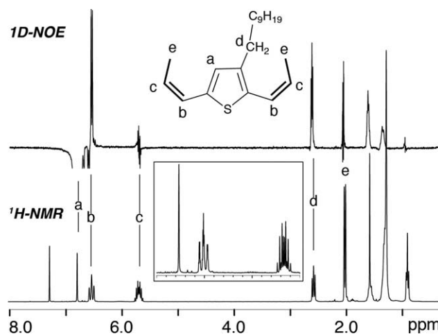
FIGURE 1 1 H NMR (bottom) and 1D-NOE (top, excited at 6.82 ppm) spectra of cis -3DTV (300.13 MHz, CDCl 3 ). Insert: magnified olefinic region.
