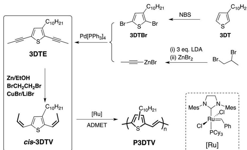
SCHEME 1 Synthesis of monomer and polymer.
