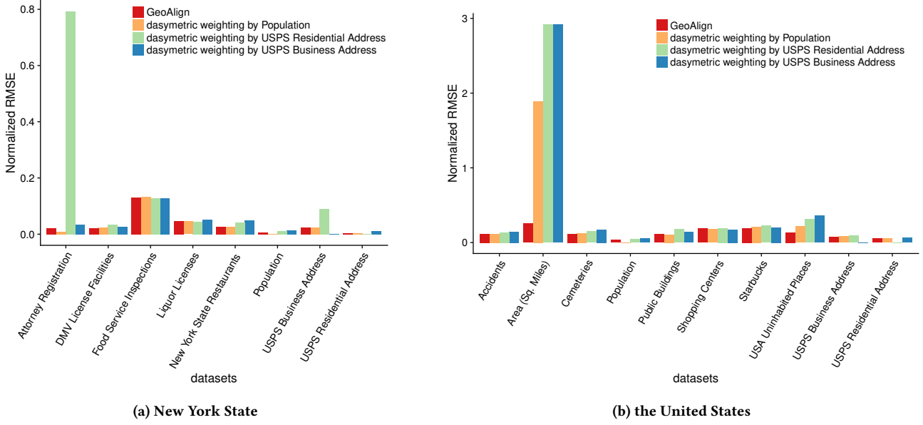
Figure 5: GeoAlign prediction performance (NRMSE) compared with dasymetric methods. Since a better prediction yields a lower NRMSE, GeoAlign is making comparable or better predictions than the dasymetric methods for tests in New York State and the United States.
