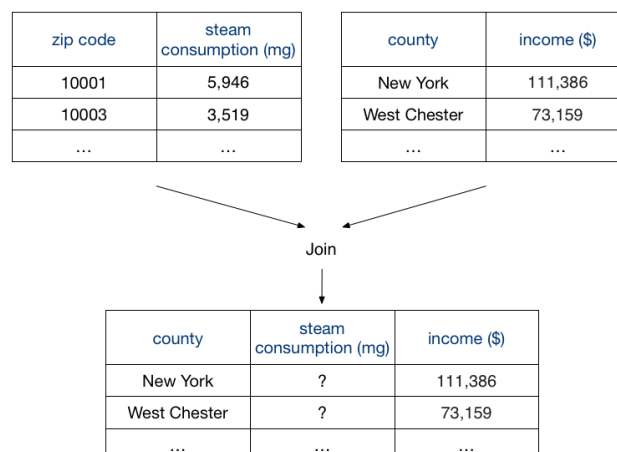
Figure 1: Join two tables for steam consumption (mg) and per capita income ($) in New York State together by county.
