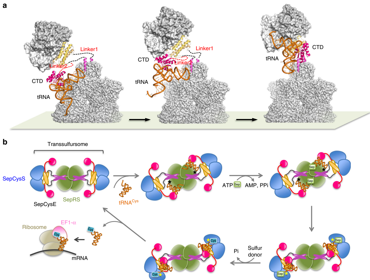
Fig. 5 Proposed mechanism of the tRNA-dependent cysteine biosynthesis by transsulfursome. a tRNA channeling for consecutive reactions of the transsulfursome. Only upper half of the transsulfursome is drawn here. (Left) The first reaction state (SepRS active form). This model was built by superposing the SepCysE(CTD)-tRNA Cys complex (present work) with the SepRS-tRNA complex (PDB:2DU3). The stretching of linker1 and linker2 allows the SepCysE(CTD)-tRNA Cys complex to reach the binding site on SepRS, while anchoring SepCysE(N-helix) to its binding site on SepRS. The anticodon of tRNA Cys is recognized by the site close to the SepCysE(N-helix) binding site. (Middle) The intermediate state. The mischarged Sep-tRNA Cys moves from the first reaction site on SepRS to the second reaction site on SepCysS without being released from bound SepCysE(CTD). Two flexible linkers of SepCysE allow the movement of Sep-tRNA Cys over this long distance. (Right) The second reaction state (SepCysS active form). The discriminator base of U73 and possibly the Sep moiety of Sep-tRNA Cys are recognized by SepCysS, followed by conversion to the canonical Cys-tRNA Cys . The anticodon of tRNA Cys may not be recognized by SepRS in this step. b A schematic drawing of the tRNA-dependent cysteine biosynthesis by transsulfursome. N-helix (purple) and NTD (orange) of SepCysE bridge the SepRS (green) and SepCysS (blue) to form ternary complex (transsulfursome) with a molar ratio of 4:4:4. SepCysE (CTD) (red) shuttles tRNA Cys between two distinct active sites on transsulfursome for sequential reactions catalyzed by SepRS and SepCysS. Each of the two enzymes recognizes tRNA Cys separately in the two steps. The released Cys-tRNA Cys is delivered to ribosome by EF1-α to finally incorporate a cysteine into proteins. Two tRNA substrates are bound to the opposite positions on transsulfursome. The recognition sites of tRNA Cys by SepRS and SepCysS are marked with black and yellow asterisks, respectively
