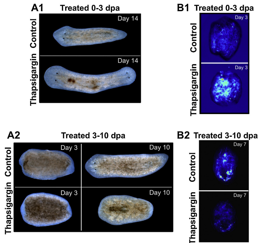
Fig. 4. \text{Ca}^{2+} Flux has Distinct Roles in Polarity Establishment vs. Tissue Remodeling. D. japonica trunk fragments treated with 1 \mu\text{M} Thapsigargin (Sigma), which inhibits SERCA-mediated ER \text{Ca}^{2+} storage, or DMSO as a vehicle control. Inhibition of ER \text{Ca}^{2+} storage from 0 to 3 days post amputation (dpa) results in (A1) double-headed regenerates due to (B1) an increase in intracellular \text{Ca}^{2+} levels, as measured by Flou-3 (Molecular Probes). Inhibition from 3 to 10 dpa results instead in (A2) a complete lack of tissue remodeling, perhaps due to (B2) depleted \text{Ca}^{2+} stores. Anterior is left for morphology ( n = 10 ), and up for Flou-3 ( n = 5 ).
