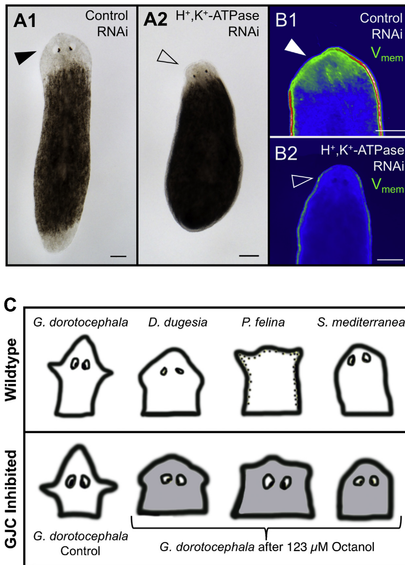
Fig. 5. Example of Shape Mutants for Investigating Regenerative Morphology. (A,B) Inhibition of the H^+,K^+-ATPase ion pump via RNAi results in (A) regenerates with shrunk heads, due to (B) ectopic loss of membrane depolarization (green) of the anterior region. V_{mem} = membrane voltage, visualized with DiBAC 4 (3) (Invitrogen). Solid arrows = normal, open arrows = abnormal. Control RNAi = VenusGFP. Anterior is up, scale bars = 200 \mu m . (C) Graphic representation of the effects of gap junction inhibition. Octanol treatment causes G. dorotocephala to regenerate with head morphologies characteristic of different species. Based on [93].
