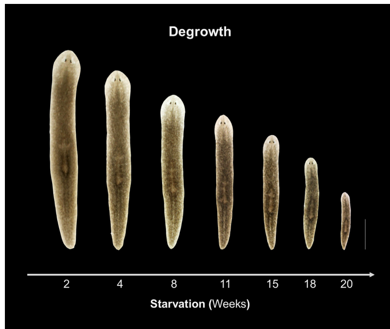
Fig. 3. Starvation-Induced Degrowth in an Intact Planarian. Tissue plasticity in planarians illustrated by a composite image of a single S. mediterranea worm over 20 weeks of starvation. Note that as the body size decreases, tissues are scaled proportionally. Anterior is up, scale bar = 1 mm.
