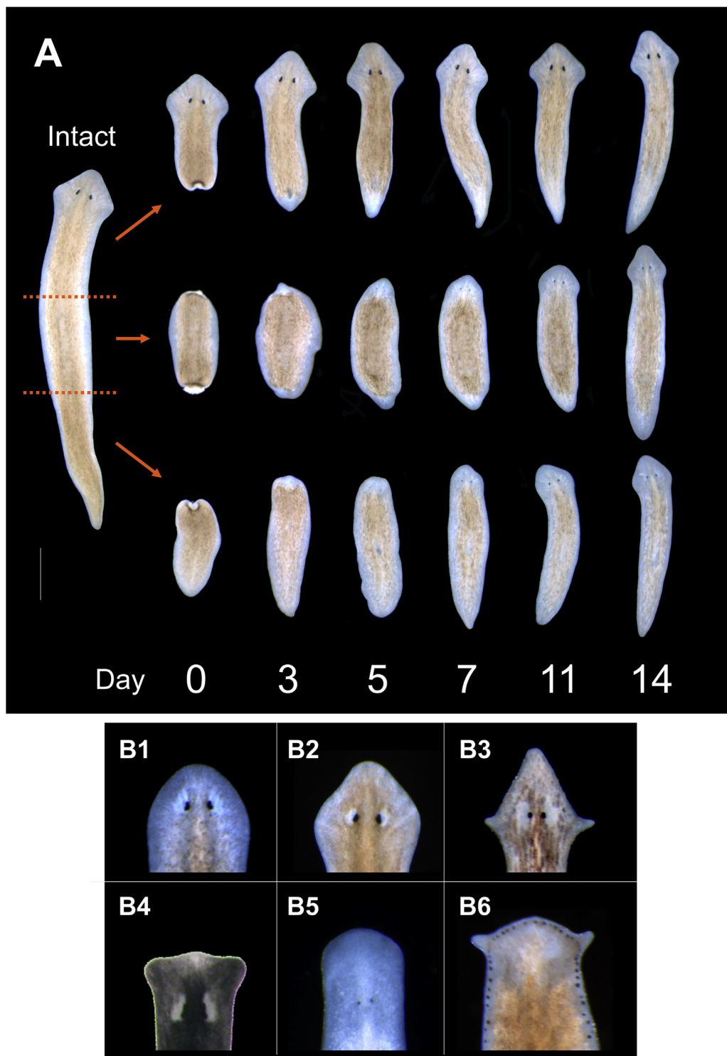
Fig. 1. Planarians as a Model for Regenerative Shape. (A) Composite image showing regeneration in a single Dugesia japonica worm over 14 days following amputation into head, trunk, and tail fragments. Anterior is up, dotted lines = amputation planes, scale bar = 1 mm. (B) Head morphologies of different planaria. (B1) Schmidtea mediterranea , (B2) Dugesia japonica , (B3) Girardia dorocephala , (B4) Phagocata gracilis , (B5) Phagocata morgani , (B6) Polycelis felina .
