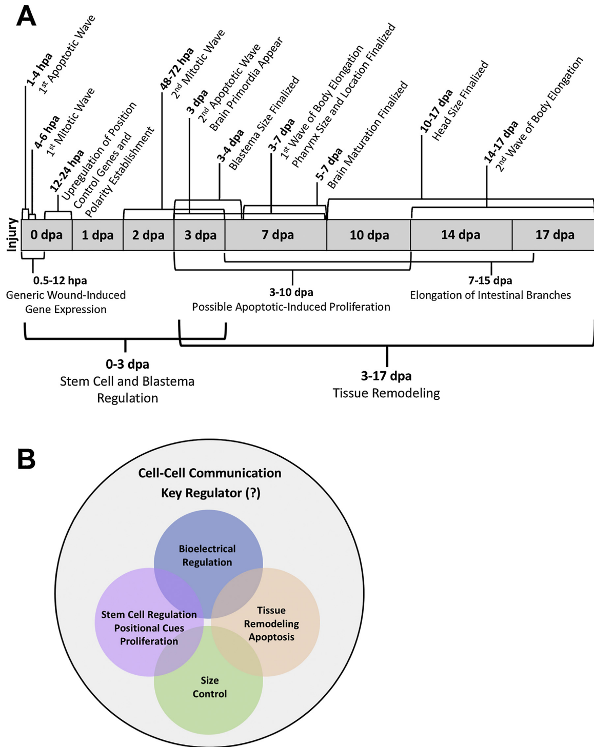
Fig. 2. The Regulation of Regenerative Shape. (A) Timeline of shape establishment events during the regeneration of trunk fragments in S. mediterranea . Based on data from [26–29,70,78,79]. Note that the timeline will be skewed for other species and/or fragment types. Hpa = hours post amputation; dpa = days post amputation. (B) Diagram of potential interactions between the central processes regulating regenerative shape during planarian regeneration.
