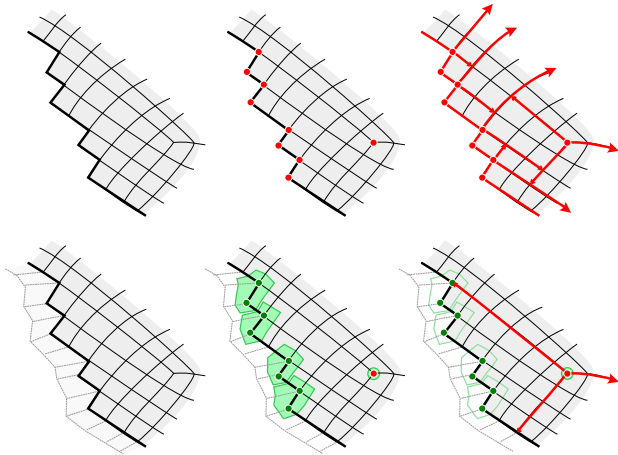
Fig. 5. Above: with the original MCG algorithm, many small patches are in presence of a jagged boundary, as in this example. Below: an example of the application of the Generalized MCG for the same input mesh. The boundary is first (virtually) expanded (left); five fenced regions (four regular, plus one degenerate of valence 3) are identified (middle), and a single patch with an open boundary is created covering the boundary (right). CC edges are not shown.
