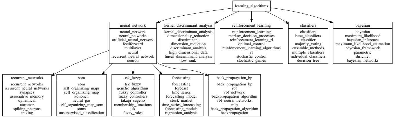
Figure 3: Parts of the taxonomy generated by TAXOGEN on the DBLP dataset. For each topic, we show its label and the top-eight representative terms generated by the ranking function of TAXOGEN. All the labels and terms are returned by TAXOGEN automatically without manual selection or filtering.
