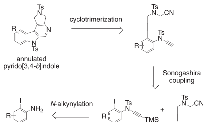
Fig. 1. Retrosynthetic analysis for annulated pyrido[3,4- b ]indoles.
