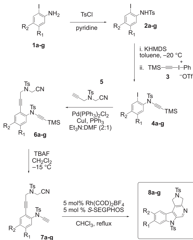
Scheme 1. Synthesis of annulated pyrido[3,4- b ]indoles via Rh(I)-catalysis.
