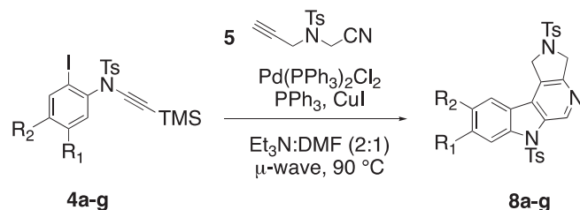
Scheme 2. One-pot synthesis of annulated pyrido[3,4- b ]indoles via Pd(0)-catalysis.
