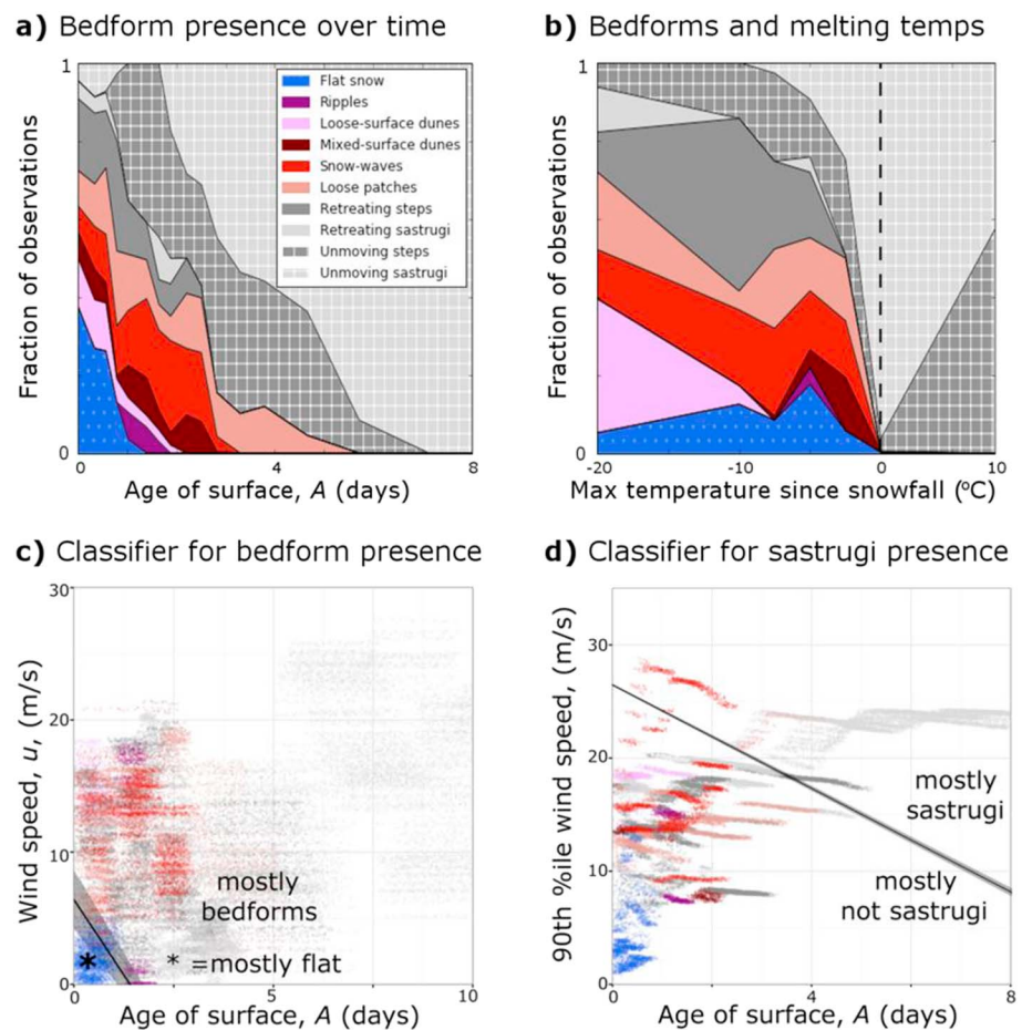
Figure 3. Bedforms on Niwot Ridge at various snow grain ages (a), temperatures (b), wind speeds (c), and 90th percentile wind speeds (d). Bedforms are color coded; see legend in plot (a). Unmoving bedforms do not move visibly in our footage. Plots (a) and (b) are one-variable frequency diagrams showing how the occurrence of various bedforms varies with the age of the snow grains and highest temperature experienced on the surface. Plots (c) and (d) are two-variable scatter plots. The lines mark the best classifiers to divide (c) flat surfaces from bedform-covered surfaces and (d) sastrugi-covered from nonsastrugi covered surfaces. Classifier uncertainties are shaded gray. Monte Carlo simulation multiplied the number of data points (section S1.4).
