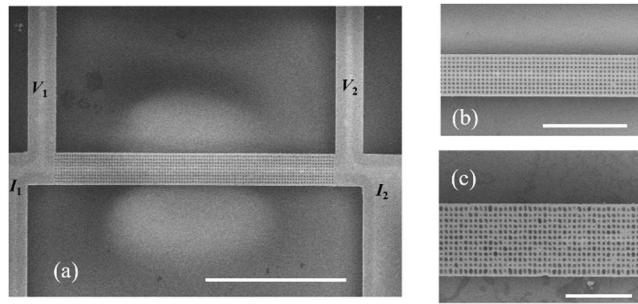
Figure 1. The SEM images of (a) suspended nanoporous Si film (diameter/pitch as 100/200 nm) with four electrical probes for thermal measurements and (b) the nanopores on this film. (c) The SEM image of the film with irregular pores over-etched from 50 nm to 94 nm in the average diameter. Scale bars are 10, 4, and 2 \mu\text{m} from (a) to (c), respectively.
