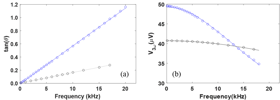
Figure 2. Frequency dependence of (a) \tan(\theta) and (b) V_{3\omega} in a typical 3\omega measurement for a nanoporous film (blue) and a solid film (black). Here symbols are measurement data and lines are for fitting.
