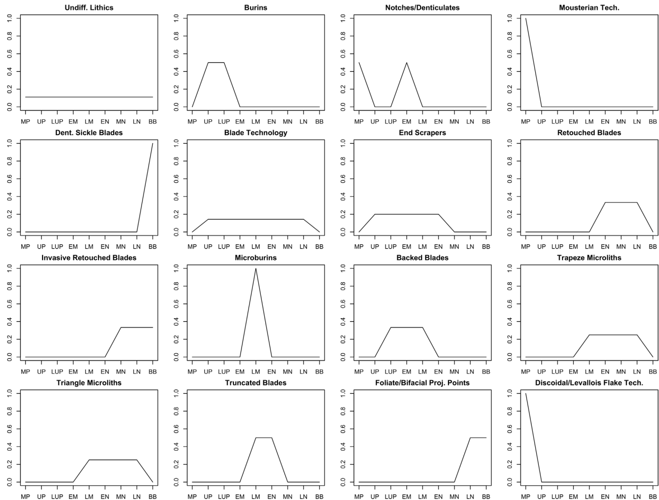
Fig. 6. Graphical representation of prior probabilities derived from the calibration dataset for the Canal de Navarrés.
