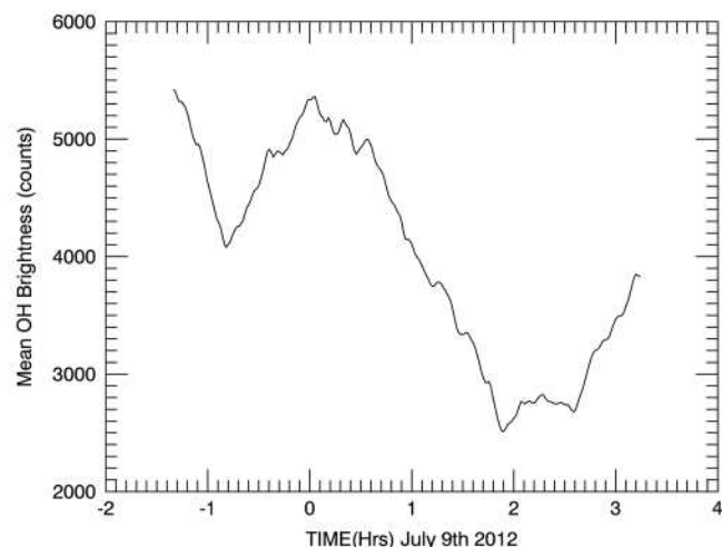
Figure 4. Plot of OH brightness from ANI data versus time in UT hours referenced to 0 h UT on 9 July 2012.
