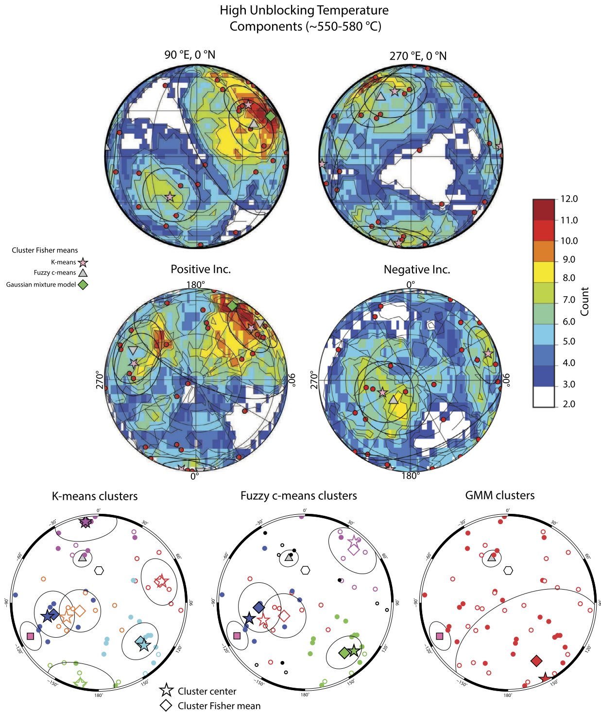
Fig. 6. Spherical contouring and cluster analysis of high unblocking temperature (HT) components. Top row: hemispherical views centered at 0°N showing the results of spherical contouring and cluster analysis. Red points show HT directions. Stars, diamonds and triangles show Fisher means of clustered directions with 95% confidence interval; pink star, k-means clustering; green diamond, Gaussian mixture model clustering; grey triangles, fuzzy c-means clustering. Contour intensity corresponds with density of directions within the counting radius for each grid node. Middle row: polar views of contouring and cluster analyses. Bottom row: equal area stereonets showing the result of clustering analysis applied to HT directions. Colors correspond with grouping assigned during clustering, for fuzzy c-means clustering, black symbols denote directions not assigned to any cluster. Open symbols, negative inclinations; solid symbols, positive inclinations. Stars show cluster centers, diamonds show Fisher mean of directions from each cluster group with \alpha_{95} confidence ellipses. Square: ~2.65 Ga unblocking temperature direction carried by Cr-Fe spinels hosted within fuchsite grains (Cottrell et al., 2016), 95% confidence ellipse shown; triangle, expected direction for ~1 Ga overprint from Warakurna intrusion (Wingate et al., 2002, 2004); hexagon, present field direction for Jack Hills.
