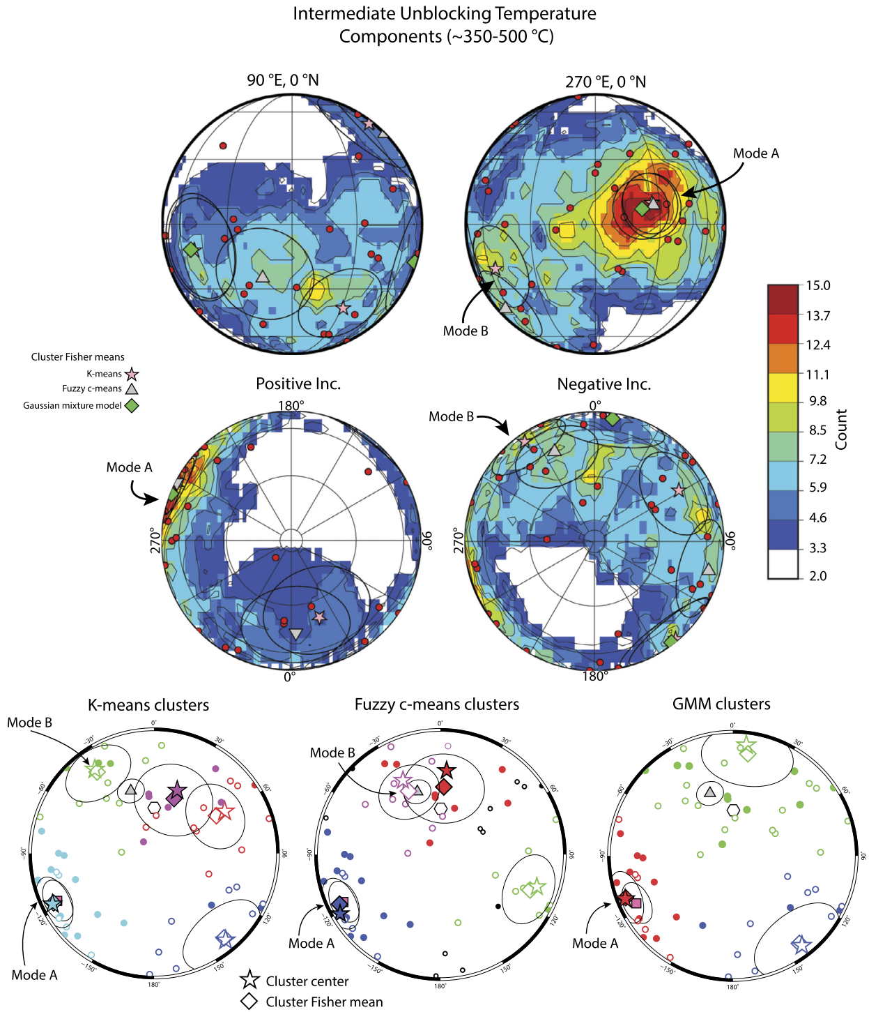
Fig. 5. Spherical contouring and cluster analysis of intermediate unblocking temperature (IT) components. Top row: hemispherical views centered at 0°N showing the results of spherical contouring and cluster analysis. Red points show IT directions. Labels identify cluster modes described in the text. Stars, diamonds and triangles show Fisher means of clustered directions with 95% confidence interval: pink star, k-means clustering; green diamond, Gaussian mixture model clustering; grey triangles, fuzzy c-means clustering. Contour intensity corresponds with density of directions within the counting radius for each grid node. Middle row: polar views of contouring and cluster analyses. Bottom row: equal area stereonets showing the result of clustering analysis applied to IT directions. Colors correspond with grouping assigned during clustering, for fuzzy c-means clustering, black symbols denote directions not assigned to any cluster. Open symbols, negative inclinations; solid symbols, positive inclinations. Stars show cluster centers, diamonds show Fisher mean of directions from each cluster group with \alpha_{95} confidence ellipses. Square: ~2.65 Ga unblocking temperature direction carried by Cr-Fe spinels hosted within fuchsite grains (Cottrell et al., 2016), 95% confidence ellipse shown; triangle, expected direction for ~1 Ga overprint from Warakurna intrusion (Wingate et al., 2002, 2004); hexagon, present field direction for Jack Hills.
