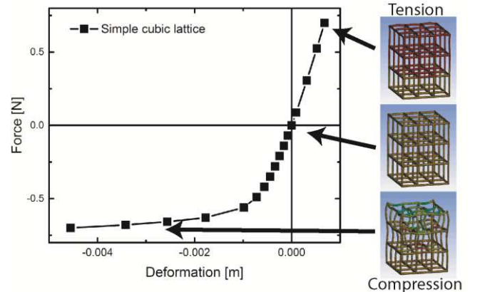
Figure 4: Representative simulated deformation of an elastomer lattice and the tensile and compressive simulated deformation of a simple cubic lattice. (from top to bottom) The simulated lattice shape at high tensile load, no load, and high compressive load.
