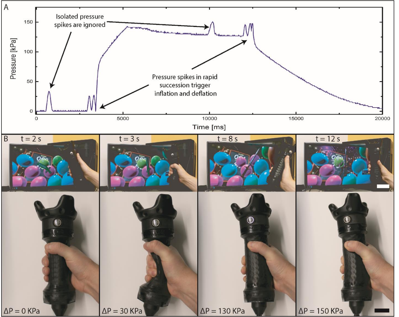
Figure 7: (A) Representative pressure profile of user-triggered inflation and deflation. (B) Sequence of demonstration interactions: [from left to right] interaction with a compliant handle corresponding to a virtual foam sword, rapid compressions of the unpressurized handle create successive pressure spike signaling to the controller to initiate a inflate the handle, interaction with the pressurized handle corresponding to a virtual metal sword, and successive compressions of the pressurized handle trigger deflation as the virtual object returns to a foam sword. Scale bars – 3 cm
