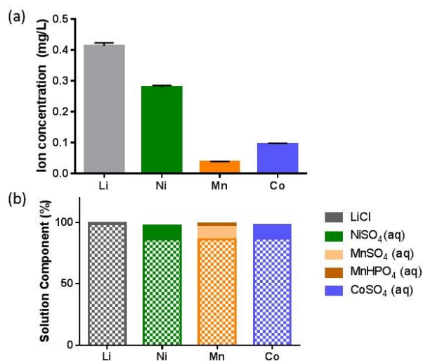
Figure 1. (a) Dissolved ion concentrations from 5 mg/L NMC suspension in B. subtilis growth minimal media over 48 hours by ICP-OES analysis (error bars are standard deviation, n = 3); (b) Speciation simulation of solution species (patterned bars indicating free ions).
