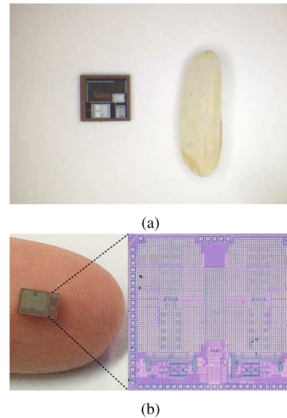
FIGURE 7. The Realized IC chips. (a) Comparison of the chip with a rice (reproduced from [85]). (b) Photo of the full-duplex transceiver IC ©CoSMIC Lab.
