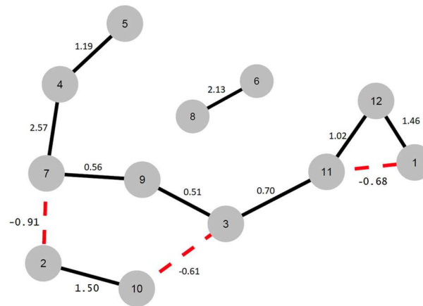
FIGURE 7. Real data: The local dependence graph of the selected FLaG-IRT model.
