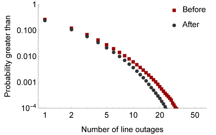
Fig. 8. Comparison of cascade size survival functions before and after upgrading critical lines in propagation simulated using the influence graph.
