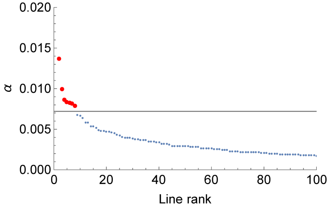
Fig. 6. \alpha_j for line j in descending order of size of \alpha_j . \alpha_j is the reduction in expected cascade size for upgrade of line j . The red dots indicate the top eight critical lines.
