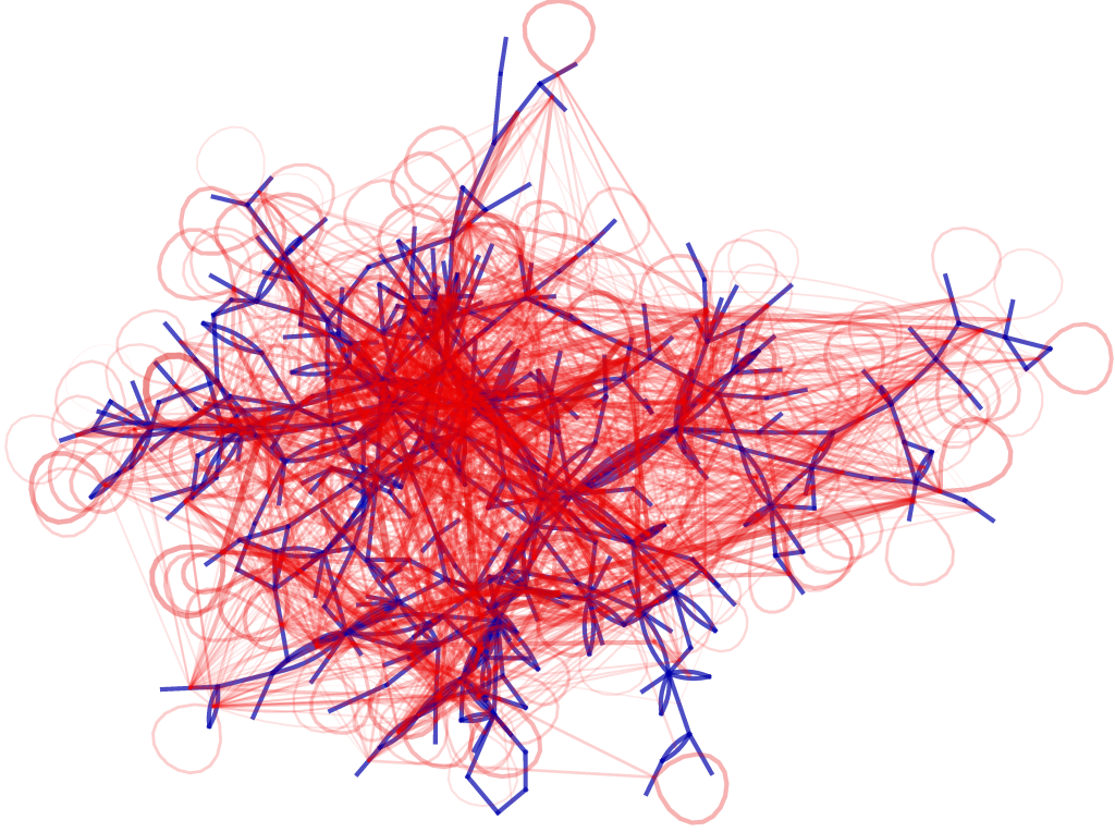
Fig. 1. The blue network is the physical utility network and the red network joining the blue lines is the influence network H_{1+} formed from the transmission line pairs in which one outage causes another. Self-loops at a node indicate lines which outage again, within the same cascade, after a time interval.
