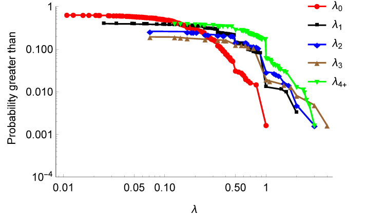
Fig. 2. Survival function of the parameter \lambda_{i,m} (the propagation and parameter for f ) for each generation m .
