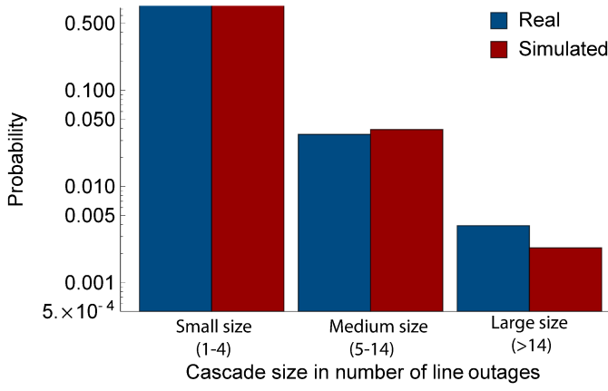
Fig. 3. Distribution of cascade sizes in three categories, binned by the number of lines failed, for real data and for the simulated data from influence graph.
