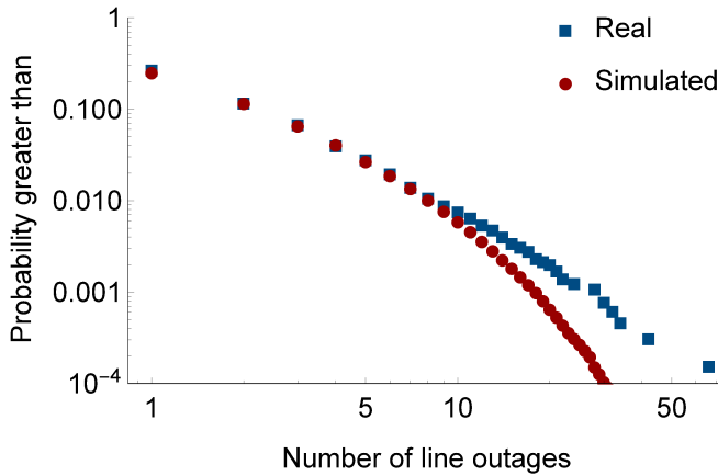
Fig. 4. Survival functions of the number of outages in each cascade for real data and for the simulated data from influence graph
