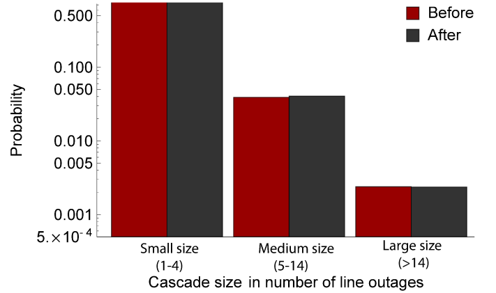
Fig. 5. Comparison of cascade sizes before and after upgrading critical lines in initial outages simulated using the influence graph. The distribution of cascade sizes does not change, but the total number of cascades decreases by about 10%.
