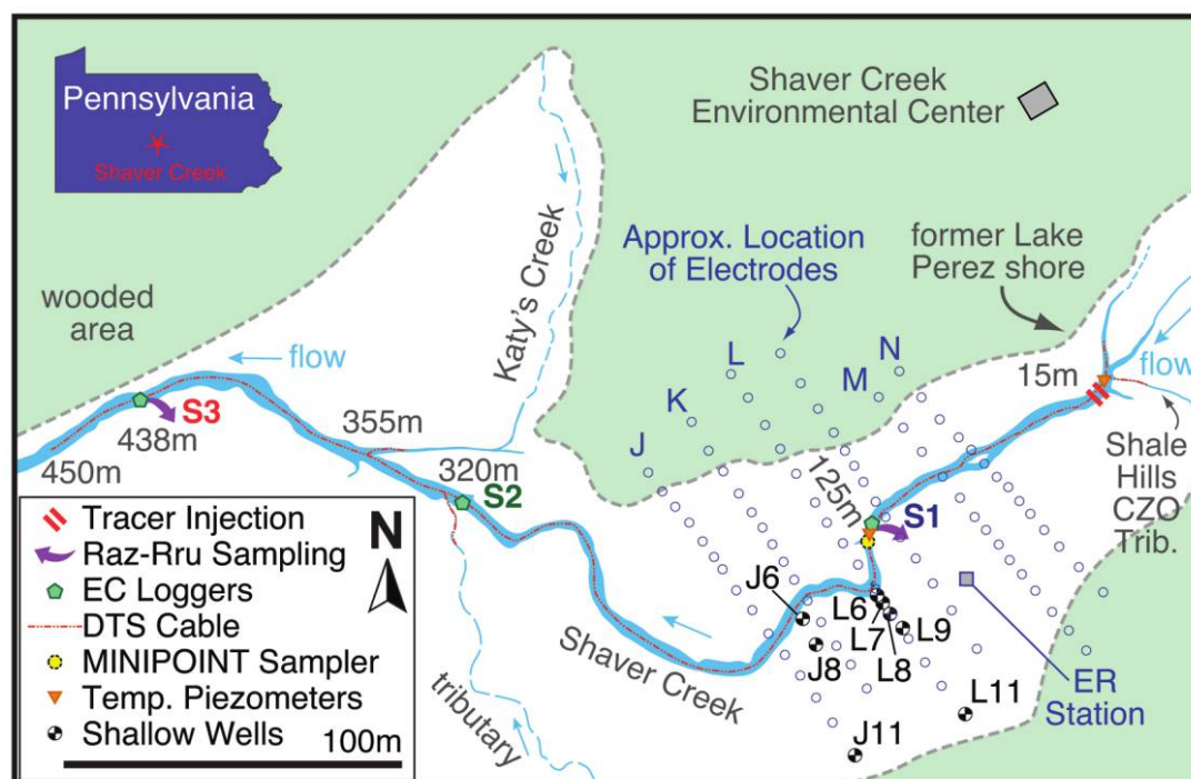
Figure 1. Field map of the 3 rd -order stream Shaver Creek. Field methods included: in-stream injections of conservative (NaCl) and reactive (resazurin [Raz] and resorufin [Rru]) solute tracers monitored in the stream (EC loggers) and in the subsurface (MINIPOINT samplers), measurement of hydraulic head (shallow wells), subsurface measurement of heat (temp. piezometers), fiber-optic distributed temperature sensing along the study site (DTS cable), and electrical resistivity imaging in select cross-sections (ER station and electrodes). Trib. = tributary, approx. = approximate.
