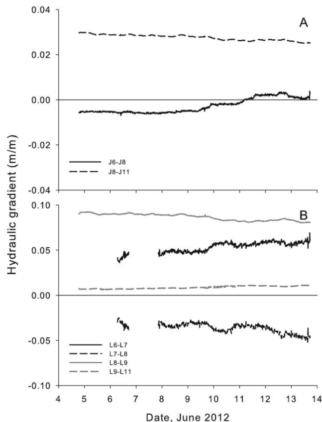
Figure 4. Time series of hydraulic gradients along the 2 well transects J (A) and L (B). J6 and L6 are adjacent to Shaver Creek, and J11 and L11 are at the distal edge of the transect, near the forest edge (Fig. 1). Gradients >0 are directed toward the stream, and <0 are directed away from the stream. Distances between wells are: J6–J8: 8.69 m, J8–J11: 34.48 m, L6–L7: 3.68 m, L7–L8: 3.19 m, L8–L9: 9.39 m, and L9–L11: 29.17 m.
