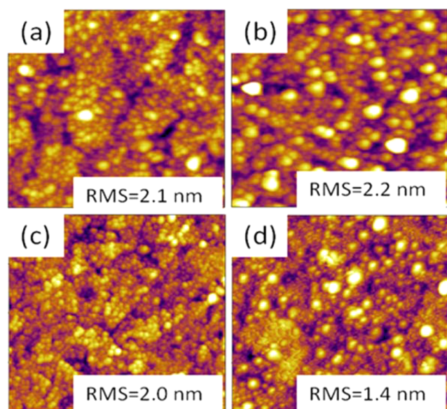
Figure 5. AFM images of \text{MoO}_x films formed on ITO substrates with different concentrations of precursor. (a) Device A, 0.02 wt %; (b) Device B, 0.05 wt %; (c) Device C, 0.10 wt %; and (d) Device D, 0.25 wt %.
