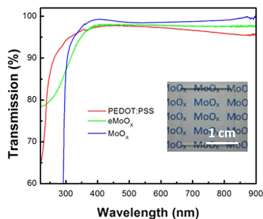
Figure 7. UV-vis transmission spectra of the \text{MoO}_x , e \text{MoO}_x , and PEDOT:PSS films; (inset) photograph of the \text{MoO}_x thin film on a labeled paper.
