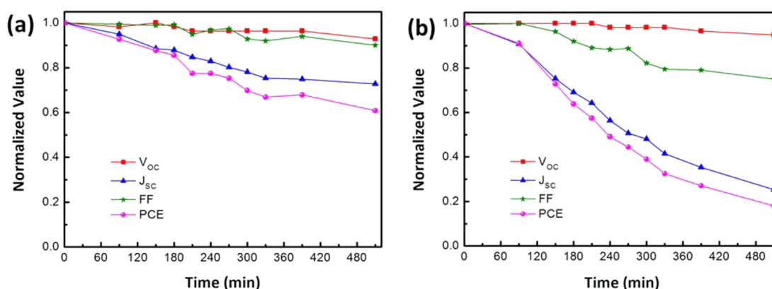
Figure 8. (a) Stabilities of key parameters in organic solar cell with MoO x prepared by polymer-assisted deposition as a hole selective layer under continuous light-illumination in air. (b) Stabilities of key parameters in organic solar cell with conventional PEDOT:PSS as a hole selective layer under continuous light-illumination in air.
