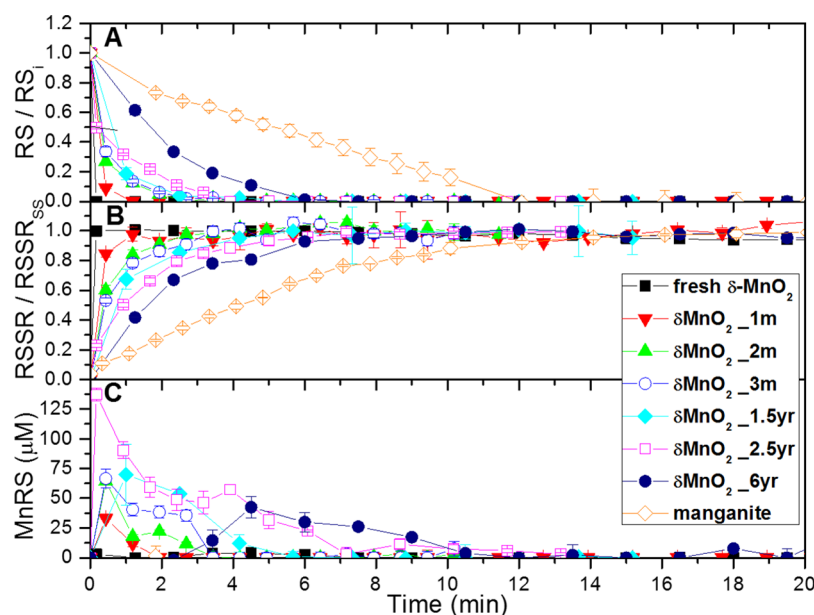
Figure 3. Temporal evolution of (A) the cysteine (CS) reactant normalized to the initial concentration of cysteine ( RS/RS_i ), (B) the cystine product (CSSC) normalized to the cystine concentration at steady state ( RSSR/RSSR_{ss} ), and (C) the intermediate sulfur surface species (MnRS) calculated from mass balance in solution during the reaction of 500 \mu\text{M} cysteine with 10 mM \delta\text{-MnO}_2 of different age or 10 mM manganite at pH 7.0. Standard deviations represent the average of at least triplicate measurements at each time point and are often smaller than the symbols.
