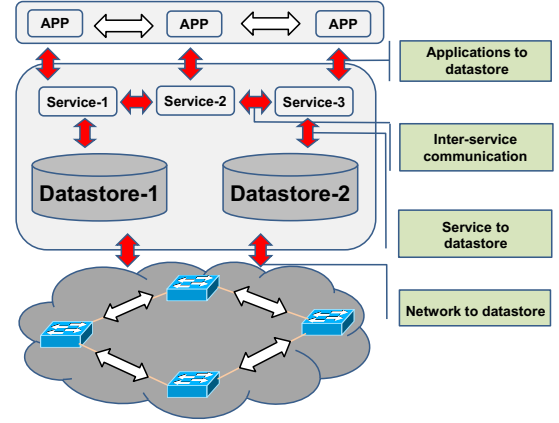
Figure 2: Threat model.
