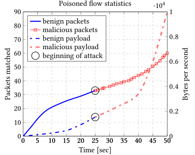
(a) Packets and payload statistics for benign and malicious traffic.
