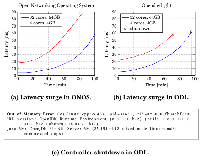
Figure 5: Flooding attack on configuration datastores.
