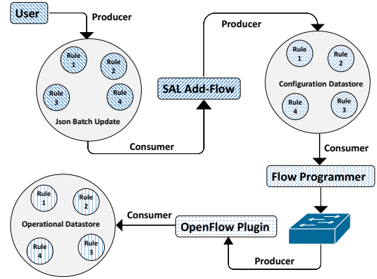
Figure 4: Ownership issues (mixed patterns show conflicts).
