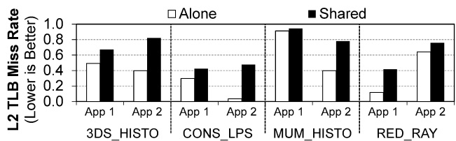
Figure 7. Effect of interference on the shared L2 TLB miss rate. Each set of bars corresponds to a pair of co-running applications (e.g., “3DS_HISTO” denotes that the 3DS and HISTO benchmarks are run concurrently).
