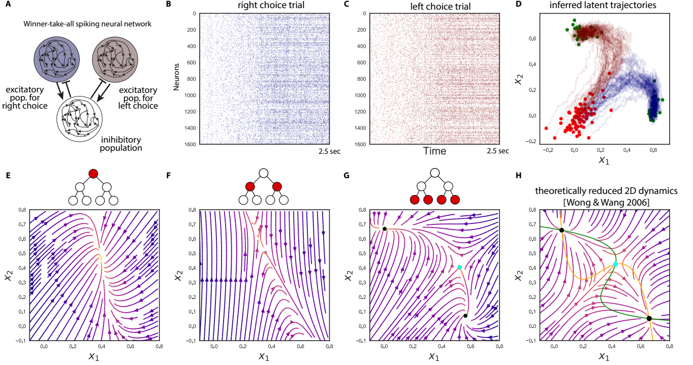
Fig. 2. TrSLDS on Winner-take-all spiking neural network. (A) Overview of the connectivity structure of the spiking neural network [9]. (B,C) raster plots of excitatory neurons for 2 random trials. (D) the latent trajectories converge to either one of the two of sinks at the end of trial (green). Each trajectory is colored by their final choice. (E-F) Dynamics captured by each level provide a multi-scale view. (H) Manual 2-dimensional reduction of the spiking neural network dynamics given the full specification [10].
