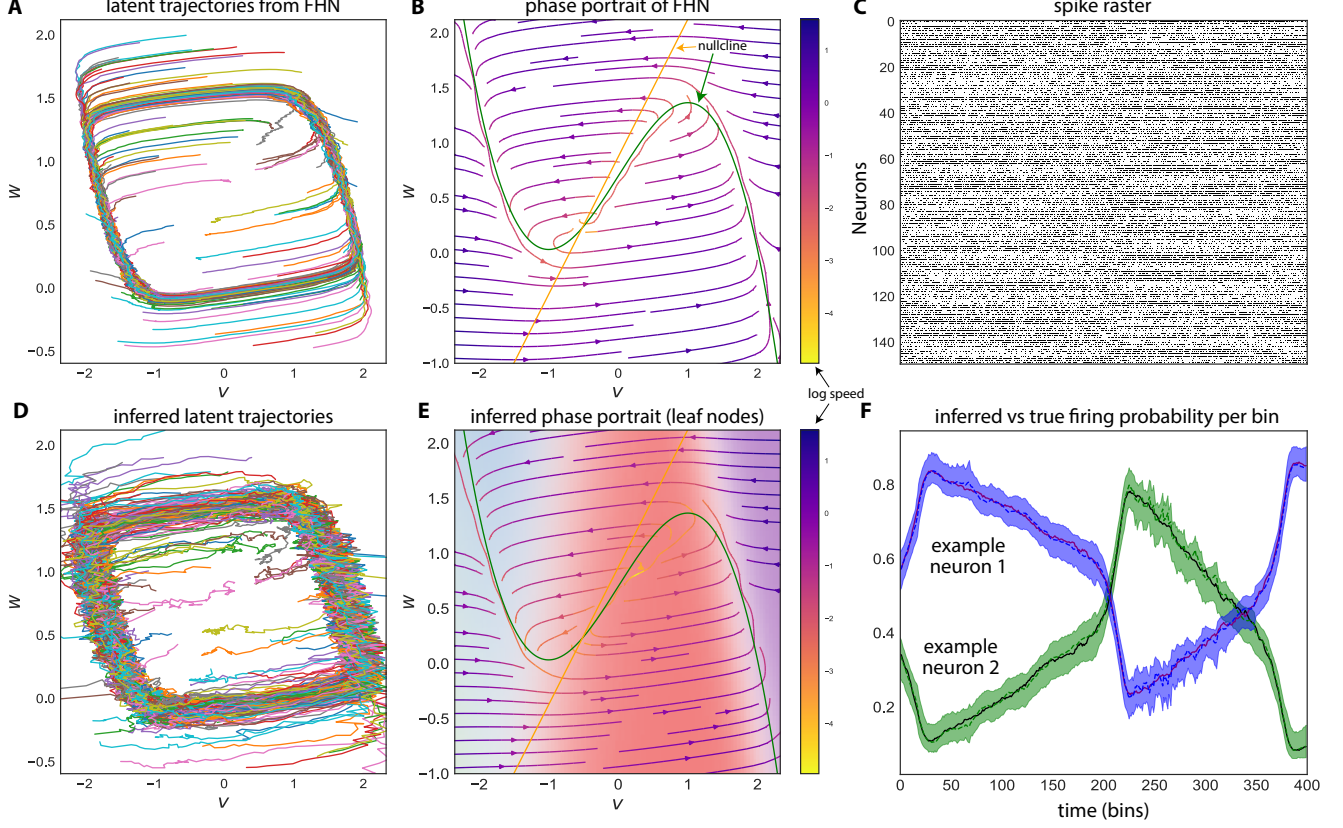
Fig. 1. (A, D) TrSLDS is able to infer the latent states. (B, E) True and learned phase portraits where the green and yellow lines are the nullclines of the system. The background color showcases the partitioning learned by the model where the darker the color is, the higher the probability of ending up in that discrete state. (C) Raster plot of a single trajectory. (F) The inferred firing rate (dotted line) and the true firing rate (solid line) are displayed for two neurons. Error bars denote \pm 3 standard deviations under the posterior.
