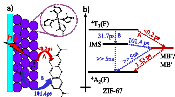
Figure 3. a) The proposed two-pathway electron transfer model in MB + -ZIF-67. b) Schematic diagram depicting energetics and time constants for electron transfer dynamics in MB + -ZIF-67.
