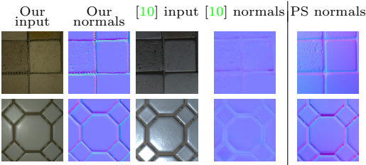
Fig. 12. Comparison of normal maps using our method and [10], with photometric stereo as reference. Even with a lightweight acquisition system, our network predicts high quality normal maps.
