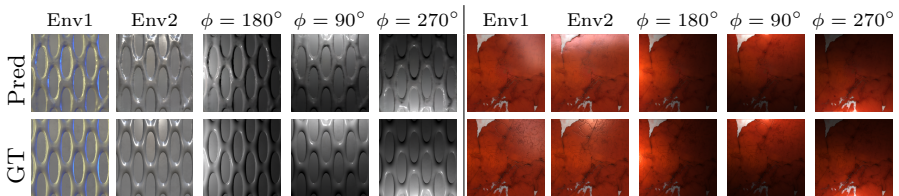
Fig. 5. Materials estimated with our method and rendered under two environment lights and three point lights (placed on a unit sphere at \theta = 50^\circ and various \phi angles).
