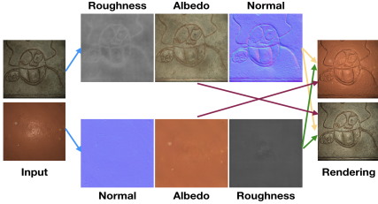
Fig. 11. A material editing example. Having reconstructed the SVBRDF and normals of the two samples, we swap the original geometry and material properties, then relight under novel illumination.
