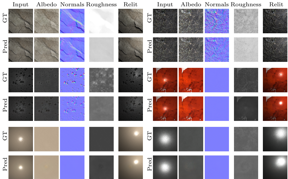
Fig. 4. BRDF reconstruction results from our full method (c1sCRF-pt in Table 3) on the test set. We compare the ground truth parameters with our reconstructions as well as renderings of these parameters under novel lighting. The accuracy of our renderings indicates the accuracy of our method.
