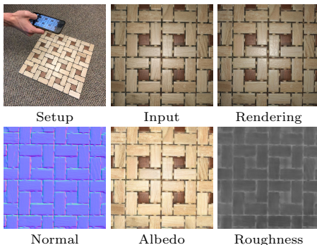
Fig. 1. We propose a deep learning-based light-weight SVBRDF acquisition system. From a single image of a near planar surface captured with a flash-enabled mobile phone camera under arbitrary lighting, our network recovers surface normals and spatially-varying BRDF parameters – diffuse albedo and specular roughness. Rendering the estimated parameters produces an image almost identical to the input image.
