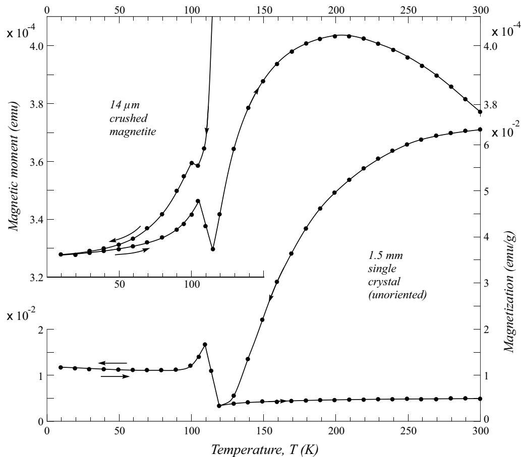
Fig. 5 Zero-field cooling and warming curves of 300-K saturation IRM for the 14 \mu\text{m} crushed and annealed magnetite sample and for a 1.5 mm natural magnetite crystal. Similar dips and recoveries of remanence are seen at T_V in these very different grain sizes of magnetite
