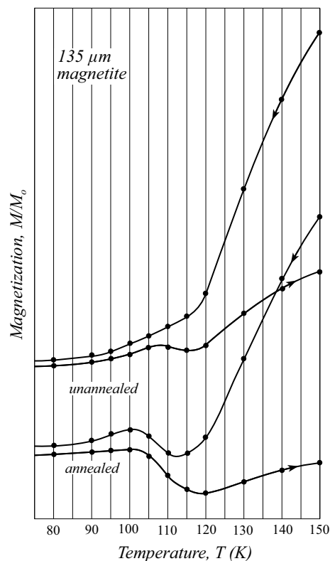
Fig. 4 Zero-field cooling and warming curves of 300-K saturation IRM for the unannealed and annealed 135 \mu\text{m} magnetites. In the unannealed samples, the remanence dip and recovery at T_V is much reduced in the warming curve and absent from the cooling curve
