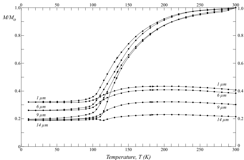
Fig. 2 Temperature dependence of saturation IRM produced by a field of 2 T at 300 K, cooled in zero field to 10 K and warmed in zero field back to 300 K for four magnetite samples. Only the 14 \mu\text{m} magnetite shows a dip and recovery of remanence at T_V ( \approx 115 K)
