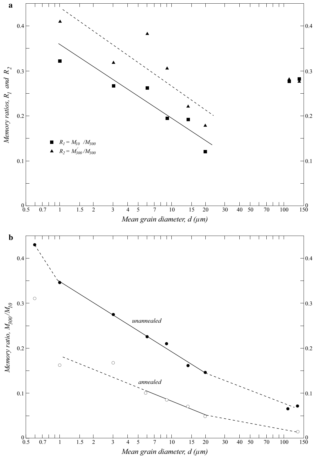
Fig. 9 Memory or remanence recovery ratios as a function of grain size for a 300-K saturation IRM cycled to 10 K and back to 300 K, and b 10-K saturation IRM cycled to 300 K and back to 10 K. In a the full-cycle ratio R_2 = M'_{300}/M_{300} is more easily measured and more practical but shows more scatter than the half-cycle ratio R_1 = M_{10}/M_{300} . Neither data trend incorporates the results for the 110 and 135 \mu\text{m} magnetites, whose room temperature memories are anomalously high. In b , the half-cycle memory ratios M_{300}/M_{10} come closer to lying on a single trend. Full-cycle ratios (not plotted) are similar to the half-cycle ratios
