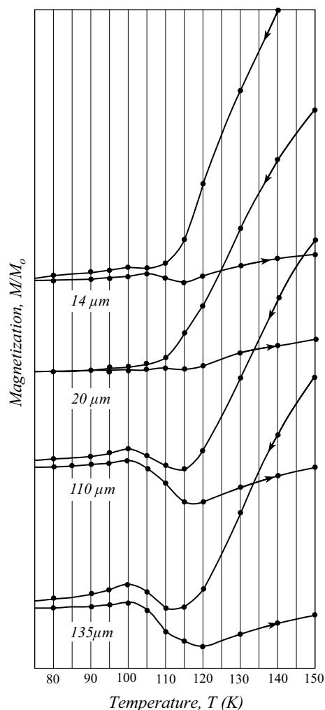
Fig. 3 Zero-field cooling and warming curves of 300-K saturation IRM over the 75–150 K interval, centered on T_V , for four larger grain size magnetites. All show a dip and recovery of remanence at T_V to varying degrees in the warming curves; the 110 and 135 \mu\text{m} samples show it also in their cooling curves
