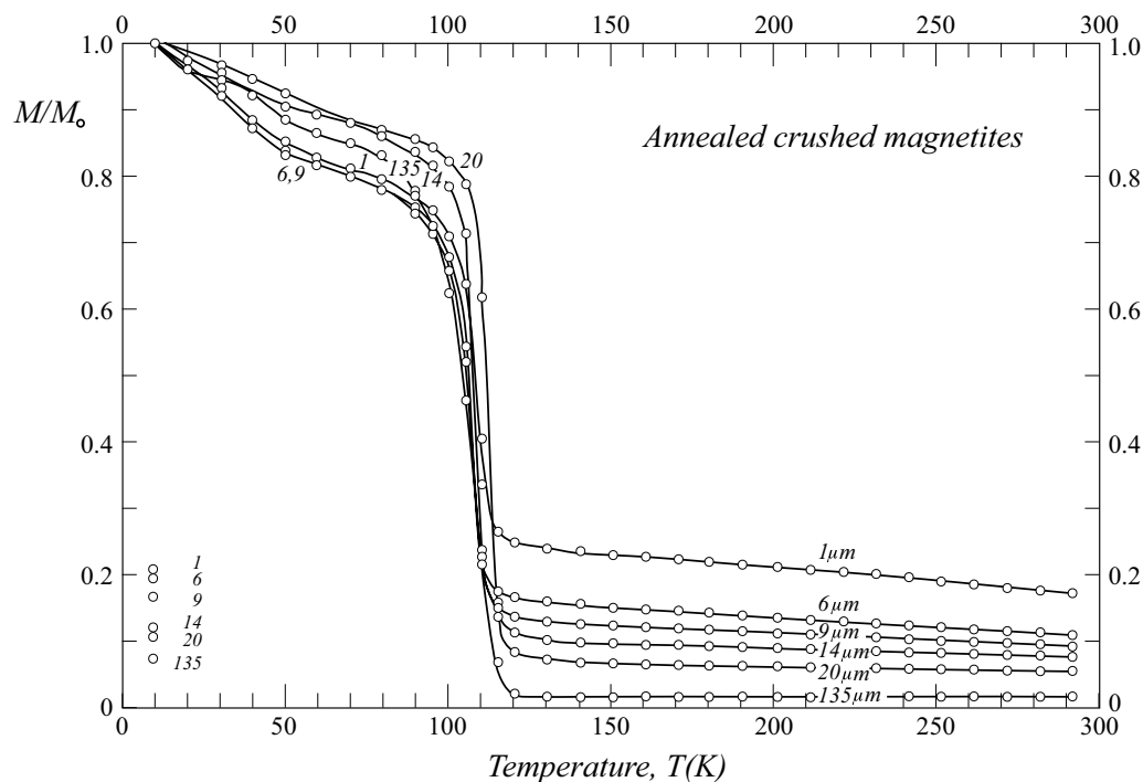
Fig. 7 Zero-field warming curves of saturation IRM produced by a field of 5 T at 10 K for six annealed crushed magnetites. Compared to the results for unannealed samples (Fig. 6), the remanence demagnetizes more between 10 and 100 K, with an inflection point at 50 K; the remanence loss at T_V is larger and more sudden; and the remanence decreases further above T_V for most grain sizes. There is substantial recovery of remanence after recooling to 10 K for the larger grain sizes
