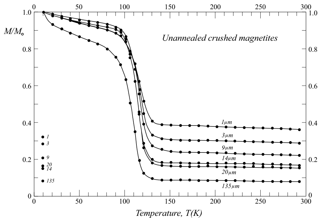
Fig. 6 Zero-field warming curves of saturation IRM produced by a field of 5 T at 10 K for six unannealed crushed magnetites. Compared to Fig. 2, the curves are rather featureless, particularly above T_V . Cooling curves were not measured but the remanences after cooling back to 10 K are shown as individual points at the left. In most cases these are virtually identical to the values measured at 300 K, indicating zero recovery of remanence in the second crossing of T_V
