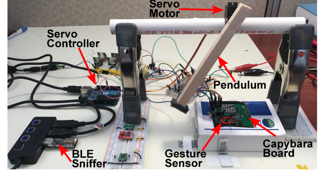
Figure 7. Experimental setup for gesture-activated remote control application.
