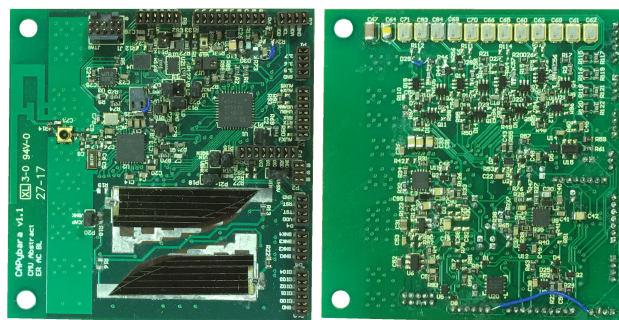
Figure 1. Cappybara hardware prototype. The solar panels, microcontroller, radio, and, five sensors are on the front side (left), and the power system with five capacitor banks and four switches is on the back side (right).
