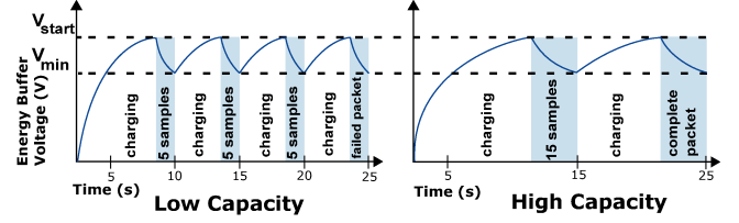
Figure 2. Execution with a fixed-capacity energy buffer. Devices are forced to trade short charge cycles for the ability to complete energy intensive tasks.
